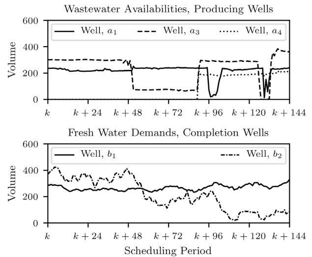
Fig. 5. Wastewater Availabilities and Fresh Water Demands for Producing Wells and Wells Undergoing Completion Respectively
