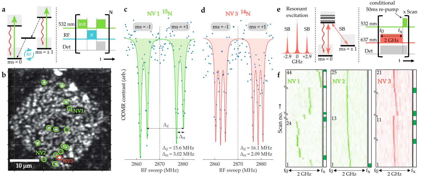
Figure 2. Correlated NV ODMR (RT) and PLE ( T < 12\text{K} ) measurements on sample A: a. Pulsed ODMR scheme utilized to identify the N isotope. Laser and radio-frequency (RF) pulses are generated by an acousto-optical-modulator and RF switch, respectively. (Laser power 0.8-1.0 mW, spot diameter \sim 800\text{ nm} .) Pulses and photon collection are triggered by a programmable pulse generator. b. Confocal PL map of the implanted region with the measured NV centers indicated by their isotope (green ^{15}\text{N} , red ^{14}\text{N} ). c. ODMR spectra for the marked NV incorporating implanted ^{15}\text{N} . d. ODMR spectra for the marked NV incorporating grown-in ^{14}\text{N} . e. Resonant excitation (PLE) scheme utilized for characterizing the optical coherence of the marked NV centers. Sidebands at 2.9 GHz are added (using an electro-optic modulator) to the scanning resonant laser to counteract optical spin pumping. Upon detection of an \text{NV}^- to \text{NV}^0 ionization event (indicated by lack of \text{NV}^- PL) a 50 ms off-resonant green re-pump is used to reset the NV charge state. f. Time traces of PLE scans measured at 10.5 K for three NV centers. Off-resonant re-pump between scans are indicated by green squares along the right column, this induces large spectral jumps in many ^{15}\text{NV} centers (e.g. NV 1). The '\!' markers along the scan axis indicate discarded scans where no NV PL is observed. The PLE traces for ^{15}\text{NV} centers typically show long periods of spectral stability between re-pump pulses.
