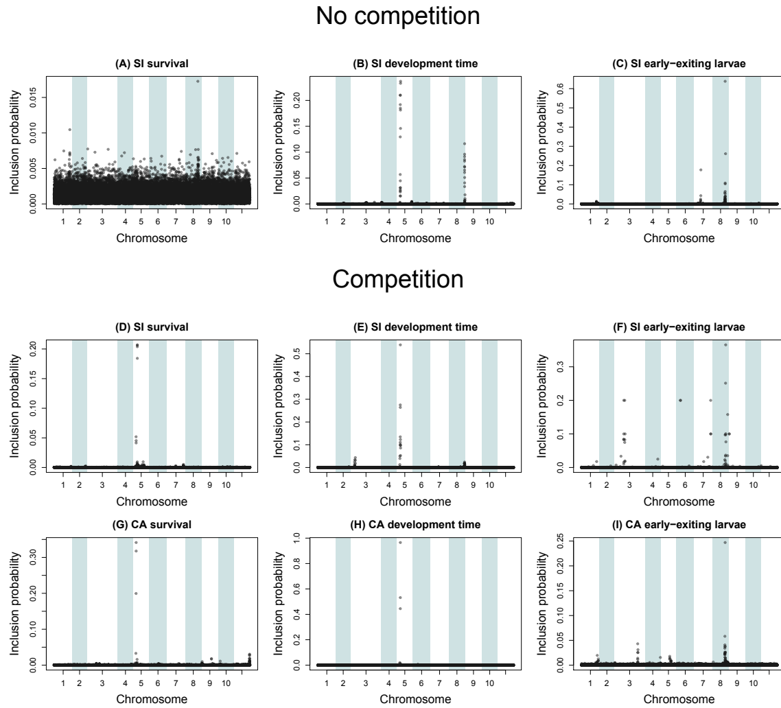
Fig. 5 Manhattan plots summarizing genotype-resistance trait associations. Points denote Bayesian posterior inclusion probabilities (PIPs) for the 32,130 SNPs. Note that the scale of the y-axis differs among panels. Results are shown for survival proportions, development time (days) and the proportion of early-exiting ("suicidal") larvae for SI with no competition (A–C), SI with competition (D–F) and CA with competition (G–I). See Fig. 6 for additional resistance traits.
