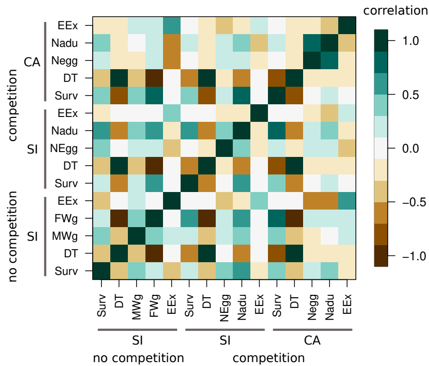
Fig. 4 Genetic correlation matrix for cowpea resistance traits. Each square denotes the Pearson genetic correlation (i.e., standardized genetic covariance) for a pair of traits computed from the output of the polygenic GWA mapping analysis. Results are shown for the SI and CA populations, and for experiments without (unshaded region) and with competition (shaded region). Traits shown are survival proportion (Surv), development time (DT), male weight (MWg), female weight (FWg), proportion of early-exiting larvae (EEx), number of eggs laid (NEgg), and number of emerging adults (NAdu).
