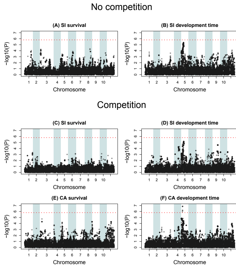
Fig. 7 Manhattan plots summarizing tests for marginal epistasis. Points denote -\log_{10}p -values for tests of marginal epistasis for each of the 32,130 SNPs. The horizontal line denotes the strict threshold for genome-wide significance, that is \frac{0.05}{32130} . Results are shown for survival proportions and development time (days) for SI with no competition (A–B), SI with competition (C–D) and CA with competition (E–F). We detected minimal evidence of epistasis for weight or total numbers of eggs or adults (not shown).
