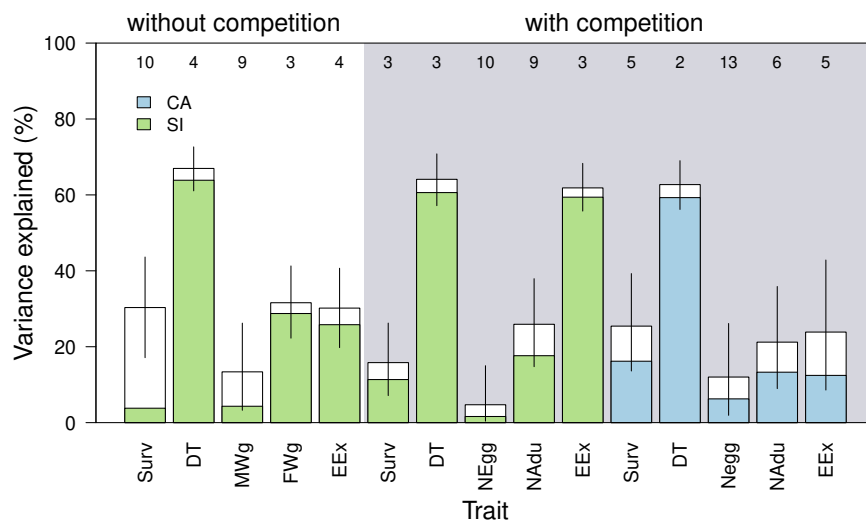
Fig. 3 Genetic contribution to resistance of cowpea RILs to C. maculatus . Bars show the percentage of trait variation attributable to additive genetic effects (PVE), and vertical lines denote Bayesian 90% equal-tail probability intervals. The shaded portion of each bar provides an estimate of the contribution of genetic variants with individually measurable effects to the PVE. Numbers along the top of the plot denote estimates (posterior medians) for the number of genetic variants causally affecting each trait. Results are shown for the SI and CA populations, and for experiments without (unshaded region) or with competition (shaded region). Traits shown are survival proportion (Surv), development time (DT), male weight (MWg), female weight (FWg), proportion of early-exiting larvae (EEx), number of eggs laid (NEgg), and number of emerging adults (NAdu).
