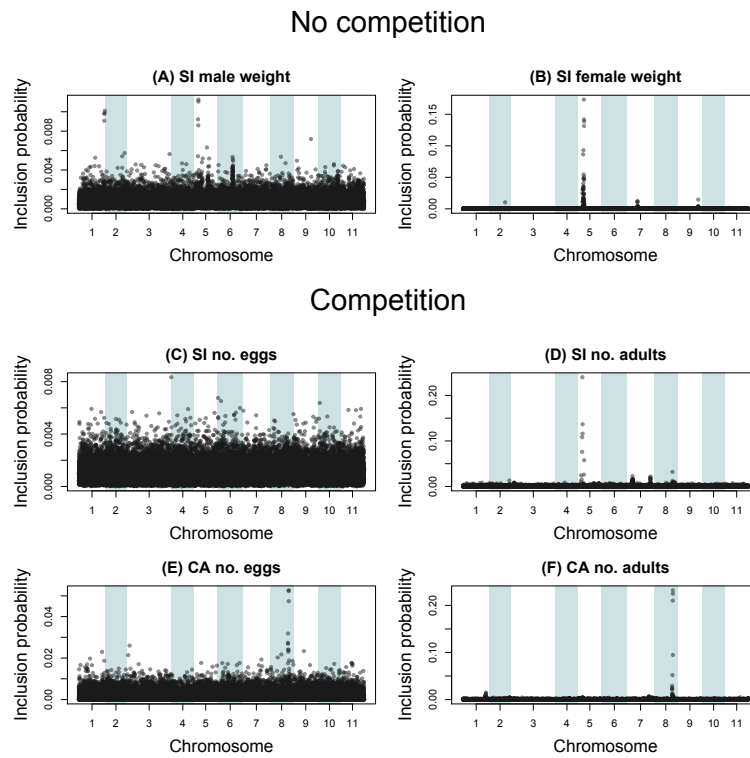
Fig. 6 Manhattan plots summarizing genotype–resistance trait associations. Points denote Bayesian posterior inclusion probabilities (PIPs) for the 32,130 SNPs. Note that the scale of the y-axis differs among panels. Results are shown for SI male and female weight (mg) without competition (A–B), number of eggs and adults in SI with competition (C–D) and the number of eggs and adults in CA with competition (E–F). See Fig. 5 for additional resistance traits.
