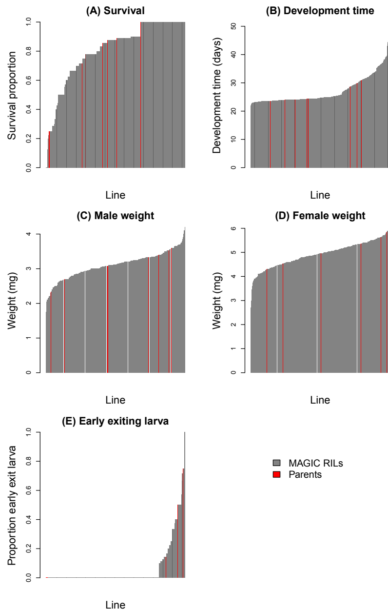
Fig. 1 Summary of resistance trait variation in the SI population under no competition (Experiment 1). Results are shown for survival (A), development time (B), weight in males (C) and females (D), and the proportion of early-exiting larva (E). Bars denote means for each line, with gray bars for the MAGIC RILs and red bars for the parents of the RILs. Lines have been sorted from smallest to largest trait values in each panel, and in panel (E) most lines had values of zero, i.e., no early-exiting larvae.
