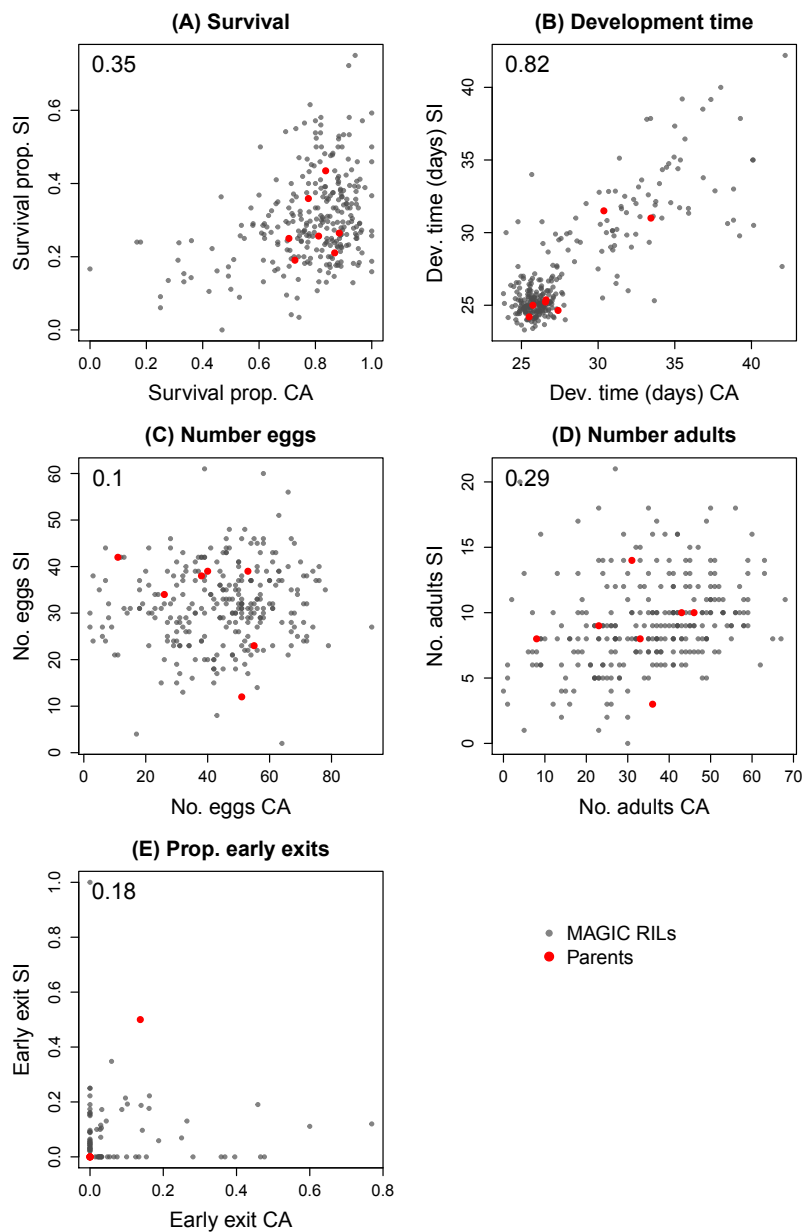
Fig. 2 Scatterplots summarizing resistance trait variation in SI and CA in the experiments that included larval competition (Experiments 2 and 3). Results are shown for survival (A), development time (B), total number of eggs laid, (C) total number of adults produced (D), and the proportion of larvae that exited seeds prematurely (E). Points denote trait values for MAGIC RILs (gray) or parents of the RILs (red). In panel (E), most lines had not early-exiting larva. Pearson correlations between populations are reported in the upper-left corner of each panel.
