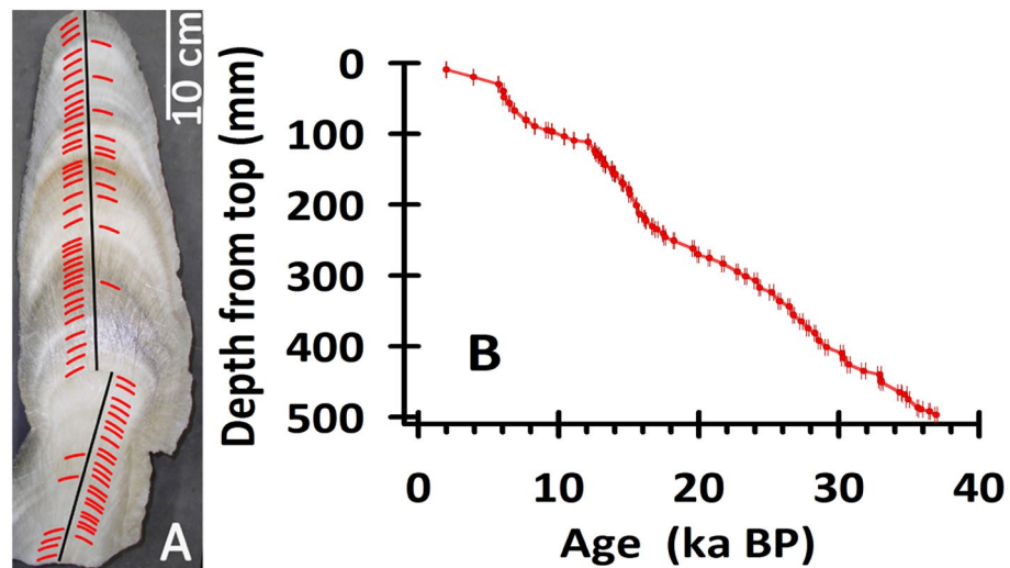
Figure 2. (A) A photograph of stalagmite FR5 from Furong Cave. The black line shows the track of the stable C/O isotopic analysis. Red markers denote the subsamples drilled for ^{230}\text{Th} dating. (B) An established age model (red line) of 67 ^{230}\text{Th} dates (red circles) with a 2-sigma uncertainty (Appendix Table 1).
