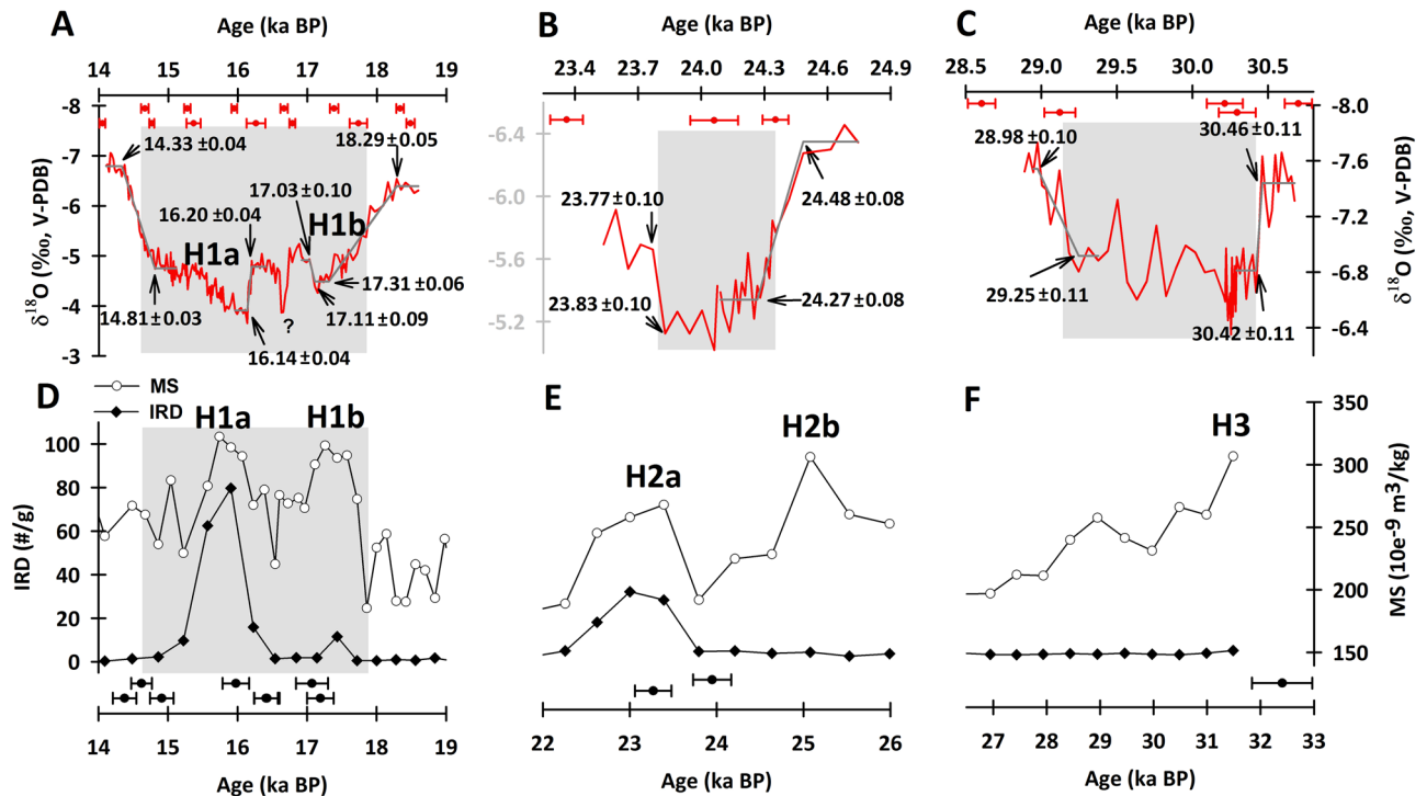
Figure 9. Stalagmite and marine records for H1, H2, and H3. (A–C) Furlong \delta^{18}\text{O} records (red) with the best fits from the RAMPFIT program 25 . ^{230}\text{Th} ages and errors are given by record. (D–F) The records of the ice-rafted detritus (IRD) (black lines with solid diamonds) and magnetic susceptibility (MS) (gray lines with hollow circles) are derived from marine sediment core SU8118 in the North Atlantic 1 . ^{14}\text{C} ages with their errors (in black) are given by record.
