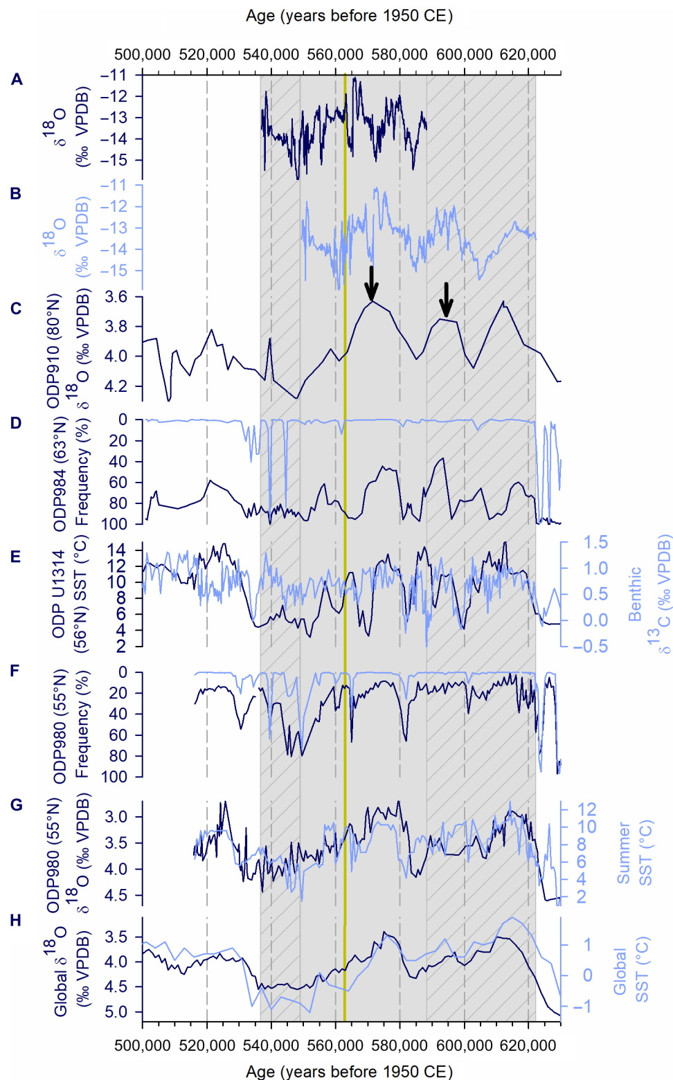
Fig. 5. Greenland speleothem \delta^{18}\text{O} record compared to marine records for the period 500 to 630 ka ago. (A) U-Th-based (dark blue) and (B) orbitally refined (light blue) age models for 80.2°N Greenland speleothem \delta^{18}\text{O} record (this study). (C) ODP 910 80°N Arctic Gateway \delta^{18}\text{O} planktic foraminifera record. Arrows indicate freshwater pulses (59). (D) ODP 984 63°N ice-rafted debris (light blue) and N. pachyderma (s.) abundance (dark blue) (45). (E) ODP U1314 56°N SST (dark blue) and benthic \delta^{13}\text{C} (light blue) (46). (F) ODP 980 55°N ice-rafted debris (light blue) and N. pachyderma (s.) abundance (dark blue) (45). (G) ODP 980 55°N benthic foraminifera \delta^{18}\text{O} (dark blue). Summer SST (light blue) (44). (H) Global benthic \delta^{18}\text{O} stack (dark blue). Stacked global sea surface temperature record (light blue) (44). Vertical gray bar highlights the area of overlapping speleothem age models, with hatched vertical bars indicating only single age models. Vertical yellow line marks the MIS 15a-14 boundary.
