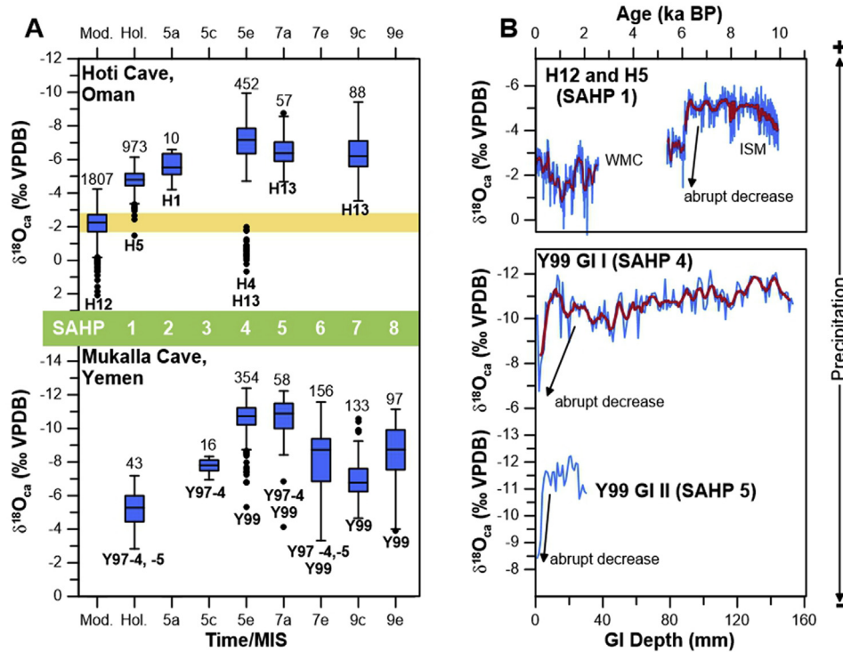
Fig. 6. (A) \delta^{18}\text{O}_{\text{Ca}} whisker-boxplot of Mukalla Cave and Hoti Cave composite records (new Y99 \delta^{18}\text{O}_{\text{Ca}} values combined with data from Fleitmann et al., 2011; Table S10). Numbers below whiskers denote sample labels and number of \delta^{18}\text{O}_{\text{Ca}} measurements. Statistically extreme values marked as black circles. (B) \delta^{18}\text{O}_{\text{Ca}} profiles of Holocene (H5 and H12), MIS 5e (Y99 GI I) and MIS 7a (Y99 GI II) stalagmites.
