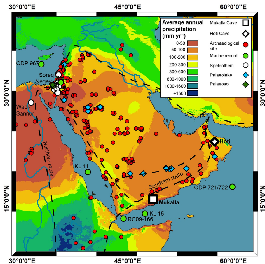
Fig. 1. Map of the Arabian Peninsula with present day (1970–2000) annual precipitation (accessible at: worldclim.org ; Fick and Hijmans, 2017). Red circles denote Middle Palaeolithic archaeological sites (Bailey et al., 2015; Breeze et al., 2015; Groucutt et al., 2015a, 2015b; Jennings et al., 2015a; Petraglia et al., 2011; Rose et al., 2011). Dashed lines show potential hominin dispersal routes (Rosenberg et al., 2011). Also shown are caves (white circles; Bar-Matthews et al., 2003; El-Shenawy et al., 2018; Frumkin et al., 1999; Vaks et al., 2010); palaeolake sites (blue diamonds; Rosenberg et al., 2011, 2012, 2013; Petraglia et al., 2012; Matter et al., 2015), marine records (green circles; deMenocal, 1995; Fleitmann, 1997; Almogi-Labin et al., 2000; Larrasoana et al., 2003; Tierney et al., 2017), lake records (blue circles; Torfstein et al., 2015) and Mukalla and Hoti caves (white square and diamond, respectively; Burns et al., 1998, 2001; Fleitmann et al., 2003b, 2011). (For interpretation of the references to colour in this figure legend, the reader is referred to the Web version of this article.)
