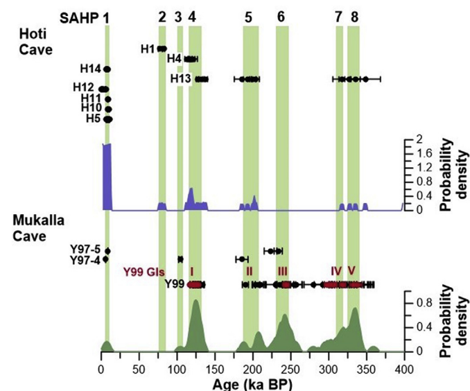
Fig. 3. ^{230}\text{Th} ages of Hoti Cave and Mukalla Cave speleothems. Red dots denote new Y99 ^{230}\text{Th} ages determined for this study. Age kernel probability density plots of Hoti (blue; 5 pt moving average) and Mukalla (green) and green bars show periods of most likely speleothem deposition. These were used to assign South Arabian Humid Periods (SAHP) 1–8. (For interpretation of the references to colour in this figure legend, the reader is referred to the Web version of this article.)
