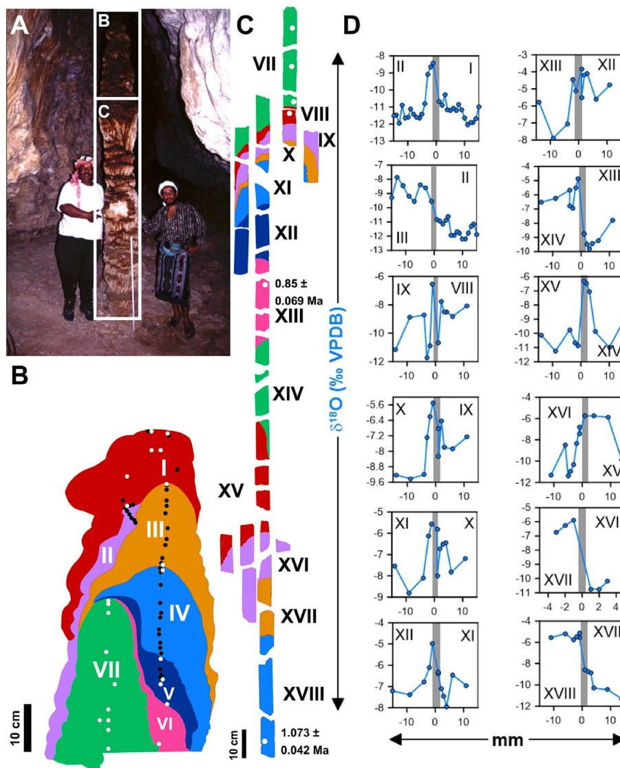
Fig. 2. (A) Stalagmite Y99 in situ in Mukalla Cave. (B and C) Y99 consecutive growth intervals (Figs. S1–S3). Location of ^{230}\text{Th} and U–Pb ages marked by black (Fleitmann et al., 2011) and white (this study) circles. (D) Plots show \delta^{18}\text{O}_{\text{Ca}} shifts over discontinuities between GIs (Tables S6 and S7).
