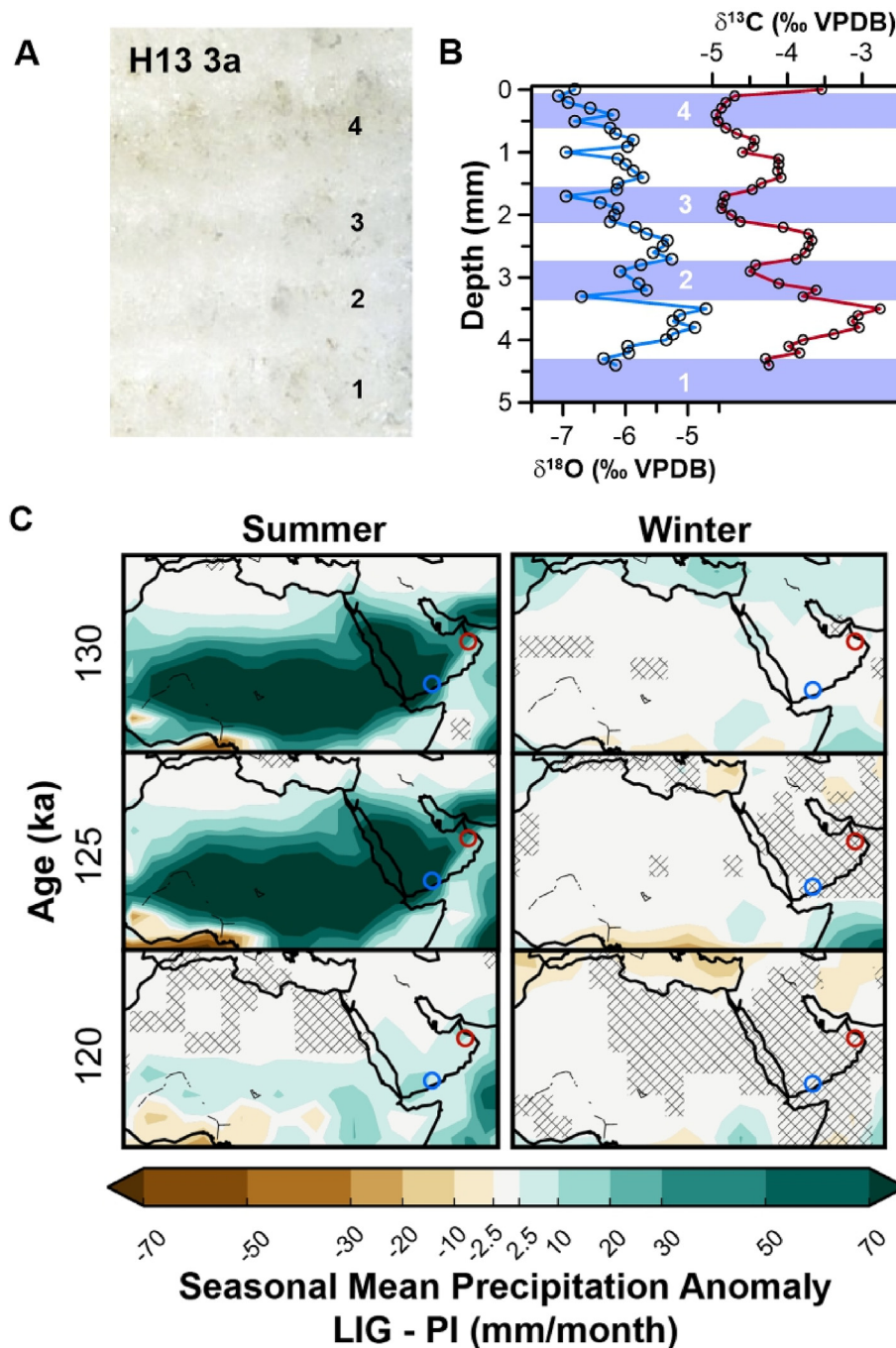
Fig. 8. (B) Sub-annual \delta^{18}\text{O}_{\text{Ca}} and \delta^{13}\text{C}_{\text{Ca}} values from a MIS 5e section of stalagmite H13 (A) from Hoti Cave (Table S8). Shaded blue areas and numbers mark the monsoon seasons. (C) Mukalla Cave (blue circle) and Hoti Cave (red circle) mapped to modelled MIS 5e winter and summer precipitation anomaly (compared to pre-industrial) (Gierz et al., 2017). (For interpretation of the references to colour in this figure legend, the reader is referred to the Web version of this article.)
