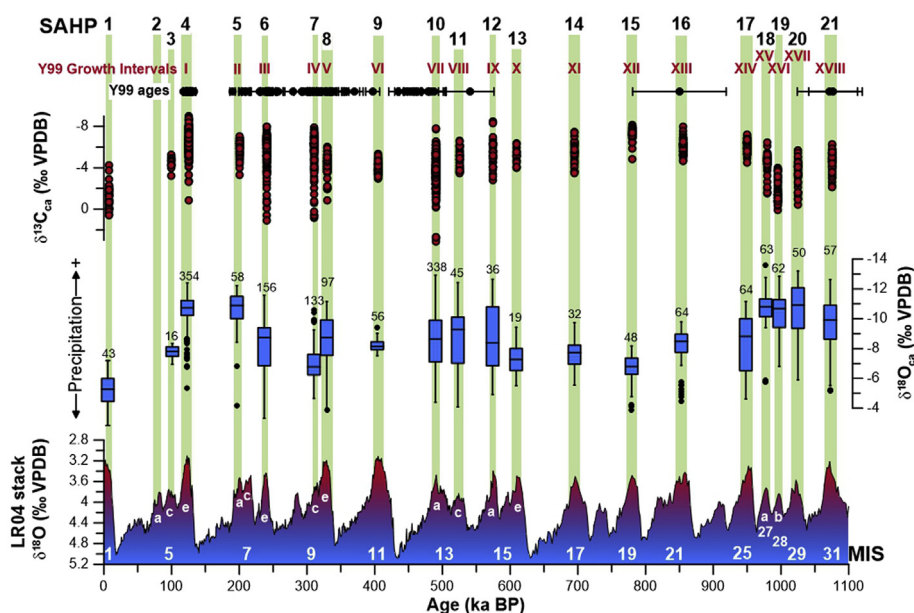
Fig. 9. ^{230}\text{Th} (Tables S1–S3) and U–Pb (Tables S4 and S5) ages for stalagmite Y99 compared to the LR04 stack \delta^{18}\text{O} record (Lisiecki and Raymo, 2005) and extended \delta^{18}\text{O}_{\text{Ca}} and \delta^{13}\text{C}_{\text{Ca}} records of Mukalla Cave stalagmites (Y97–4, Y97–5 and Y99). Undated Y99 growth intervals were assigned to intermediate interglacials and warm substages. Green bars denote timing of SAHPs (South Arabian Humid Periods). Marine Isotope Stages follow the taxonomy of Railsback et al. (2015). (For interpretation of the references to colour in this figure legend, the reader is referred to the Web version of this article.)
