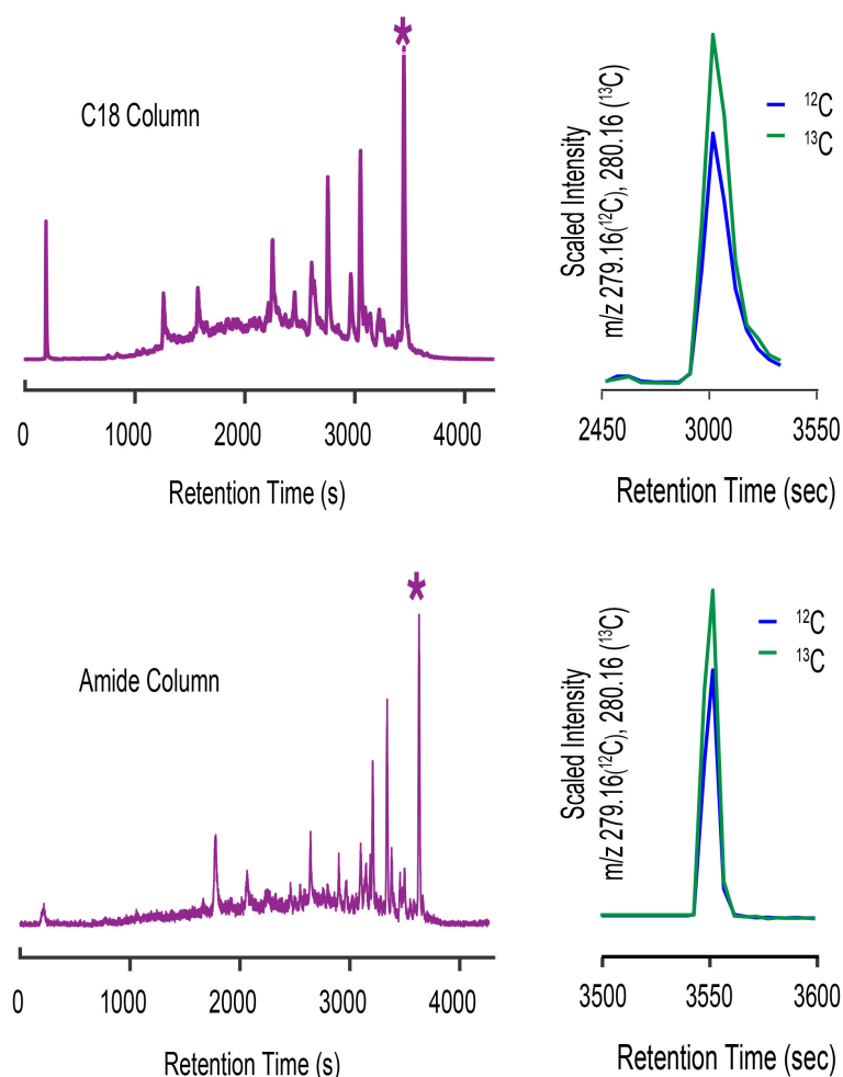
FIGURE 11 | LC-ICPMS ^{127}\text{I} -chromatogram of organic iodine metabolites in spent media from a culture of Prochlorococcus MIT9215 separated on a C18 column ( top, left ) and an amide column ( bottom, left ). The complex mixture of organic iodine metabolites shown in the chromatograms is typical of culture media and seawater samples. When the ESIMS data of the starred (*) peak from each analyses are processed with CMA-T and CMA-C we only find one target ion at 279.16 D ( top and bottom, right ) that is common to both datasets.
