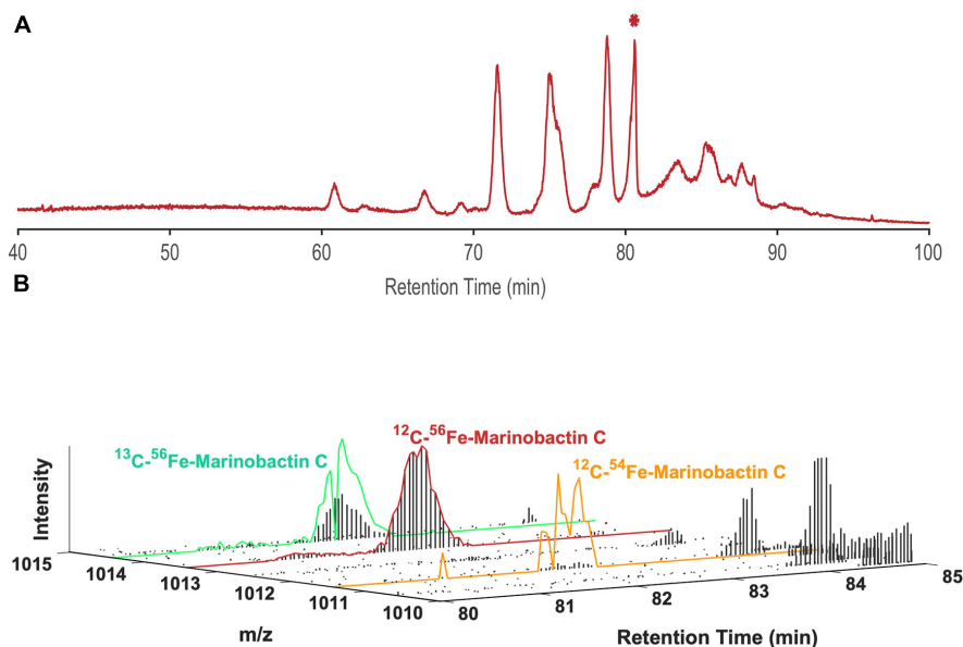
FIGURE 1 | (A) LC-ICPMS ^{56}\text{Fe} -chromatogram of dissolved organic matter collected by SPE from the North Pacific Ocean. Each discrete peak represents one (or a combination of multiple) Fe-containing organic compounds. The starred peak (*) at 80.6 min was selected as our target for characterization, and (B) LC-ESIMS data between 80–85 min and 1010.00 D–1015.00 D for the same sample. Using the isotope ratio search algorithm with \Delta m = 1.995 D and R = 15.7 for ^{54}\text{Fe} and ^{56}\text{Fe} the peak at 80.6 min was assigned the m/z of 1013.44 D. It is then identified as marinobactin C (EIC outlined in red), by comparison of its exact m/z with a catalog of known siderophores. The scaled plots for ^{54}\text{Fe} -1011.45 D, and ^{13}\text{C} - ^{56}\text{Fe} -1014.44 D of marinobactin C are outlined in orange and green respectively. Each vertical black bar represents the ion intensity at each mass in a scan at a given retention time.
