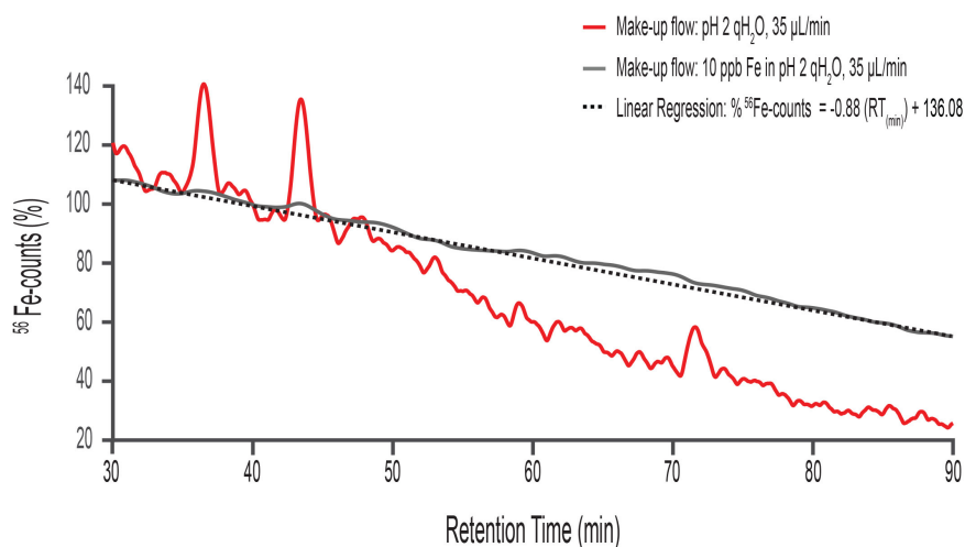
FIGURE 4 | LC-ICPMS ^{56}\text{Fe} -chromatogram of ferrichrome and ferrioxamine E (200 fmol each), with a make-up flow of 35 \mu\text{L}/\text{min} pH 2 qH 2 O (red trace). To measure the effect of solvent B on the detection of iron, we performed an identical analysis, but added 10 ppb ^{56}\text{Fe} to the make-up flow (gray trace). Iron delivered to the ICPMS in this analysis was dominated by the 10 ppb infusion and was effectively constant over time, making the ^{56}\text{Fe} counts a good proxy of Fe sensitivity by ICPMS. A linear regression of ^{56}\text{Fe} -counts and time (black solid dashed line) gives a good fit to the data with \% \text{Fe} = -0.88 (\text{retention time (min)}) + 136.08\% with r^2 = 0.99 . For the comparison here, each ^{56}\text{Fe} -chromatogram, was normalized to the ^{56}\text{Fe} counts at 40 min, the average retention time of the two standards.
