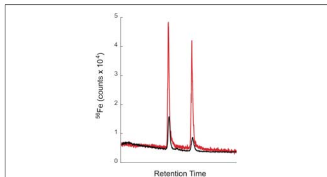
FIGURE 3 | LC-ICPMS Fe chromatograms of ferrichrome and ferrioxamine E (2 nmol each) showing the better sensitivity and decreased solvent effects of the low-flow/make-up flow system (red trace) compared to the high-flow/split system (black trace). The low flow/make-up flow system was eluted with a flow rate of 10\text{ }\mu\text{L}/\text{min} with a make-up flow of 35\text{ }\mu\text{L}/\text{min} pH 2 \text{qH}_2\text{O} . The high-flow/split system was eluted with a flow rate of 200\text{ }\mu\text{L}/\text{min} , which was split post-column with, 20% entering the ICPMS, 80% going to waste.
