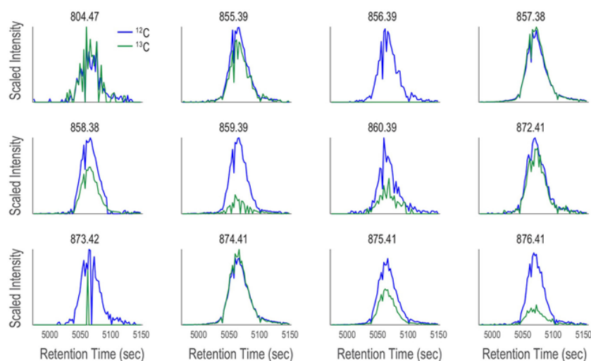
FIGURE 7 | Twelve target ions discovered by CMA-T that elute within T_w = 4973-5153 s in the SPE organic extract of V. cyclitrophicus strain 1F-53 culture media after addition of iron. The EIC of each target ion (M; blue traces) is overlaid with the EIC of (M+1.003; green traces), after scaling the latter by the relative abundance of ^{13}\text{C} calculated according to Figure 8 , under the assumption of a singly charged ion and 50% carbon content.
