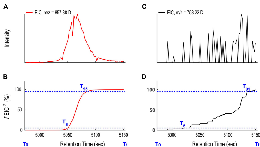
FIGURE 6 | Illustration of the compound mass assignment-time (CMA-T) algorithm. (A) The ion at 857.38 D targeted by CMA-T has the rise and fall in intensity with time expected for a well-shaped peak eluting from the LC. (B) The integral of the square of the 857.38 D ion intensity ( I^2 ) over time \Delta T ( T_{95}-T_5 ) rises from 0.05% ( T_5 ) to 0.95% ( T_{95} ) of its total value in \Delta T \leq 0.2T_w . (C) Ions that arise from noise show a more gradual rise and fall in intensity over time, and (D) for the same \Delta T , the integral of I^2 between T_5 to T_{95} \geq 0.2T_w . The comparison between \Delta T ( T_{95}-T_5 ) and 20\% T_w is used as a filter to differentiate target ions from noise.
