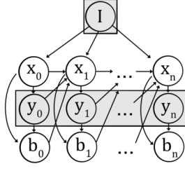
Figure 3: The design process described in Figure 2 can be represented as a Dynamic Bayes Net. Each design, x_t , is dependent on the previous design, x_{t-1} , and its outcomes, y_{t-1} , the designer’s intentions, I , and the state of the designer’s beliefs, b_{t-1} . The design and its outcomes influence the state of the designer’s beliefs about the design space.
