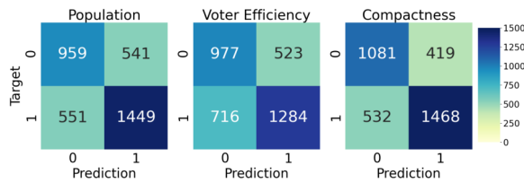
Figure 7: These confusion matrices show the frequency with which the model predicted the designer’s intentions towards a specific outcome.
