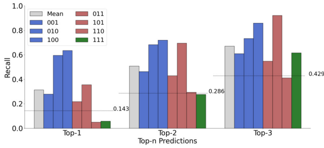
Figure 6: This plot shows the frequency with which the classifier predicted all three of the design intentions for each class, color-coded by the number of intentions, within the top one, two, and three most probable classes. The dotted lines show the threshold of random chance for each of these and the mean across classes for each group is shown in gray.
