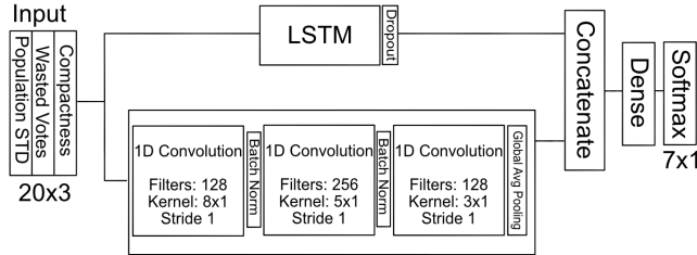
Figure 4: We classified design intentions from observed outcomes using an LSTM-FCN architecture adapted directly from [14]. The input to the network is a 20-step sequence of design outcomes; the output is a probability over the seven possible combinations of design intentions.
