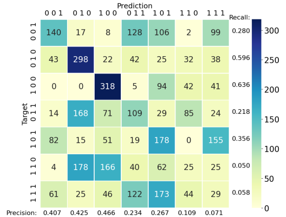
Figure 5: This confusion matrix shows prediction frequency for each subset of design intentions, represented as binary masks over [balance population, improve voter efficiency, maximize compactness]. For example, 101 represents intentions to balance population and maximize compactness.
