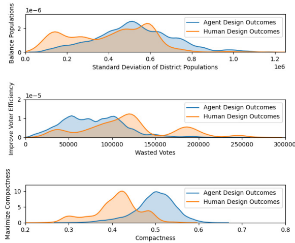
Figure 8: Density plots of relevant raw design outcomes for each intention, as explored by agent and human designers, suggest that, while humans found designs with more balanced populations, the agent tended to be more effective at improving voter efficiency and maximizing compactness.
