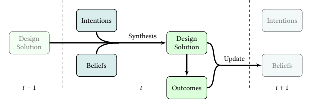
Figure 2: Each new design solution is synthesized from the current design based on the designer's intentions and beliefs about the design space. Beliefs are updated based on how the current solution affects observed outcomes.
