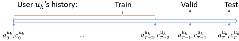
Figure 2: Data split
