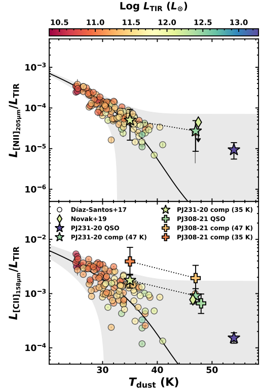
Fig. 6. [\text{NII}]_{205\text{ }\mu\text{m}} and [\text{CII}]_{158\text{ }\mu\text{m}} line deficits (top and bottom panel, respectively) with respect to the total IR luminosity ( L_{\text{TIR}}(8\text{--}1000\text{ }\mu\text{m}) ) for quasars PJ231–20 and PJ308–21 and the companion galaxies and the LIRG sample of Díaz-Santos et al. (2017) as a function of dust temperature and color-coded by \log L_{\text{TIR}} . We also report the measurements obtained for the z = 7.54 quasar ULAS J1342+0928 (Novak et al. 2019). The sources in system PJ231–20 are indicated by stars, and those in system PJ308–21 are marked with crosses. For the companion galaxies we report the cases with assumed dust temperatures of 47 K and 35 K. These points are connected by a dashed line. The solid lines are the best fit to the LIRG sample performed in Díaz-Santos et al. (2017) using the model L_{\text{line}}/L_{\text{FIR}} = \epsilon_0 \exp(-S_{63}/S_{158})/\delta with (\epsilon_0, \delta) = ((1.26 \pm 0.16) \times 10^{-3}, 0.50 \pm 0.04) for the [\text{NII}]_{205\text{ }\mu\text{m}} line, and (\epsilon_0, \delta) = ((14.0 \pm 0.9) \times 10^{-3}, 0.68 \pm 0.04) for [\text{CII}]_{158\text{ }\mu\text{m}} line. We scaled the best fits by a constant factor because different FIR luminosity definitions were employed by Díaz-Santos et al. (2017). The best-fit scaling values are 0.56 for [\text{NII}]_{205\text{ }\mu\text{m}} line and 0.44 for [\text{CII}]_{158\text{ }\mu\text{m}} line. The gray shaded area represents the 1\sigma scatter of the relation. The Novak et al. (2019) points were slightly shifted along the dust temperature axis (assumed to be 47 K) for a better visualization of the data.
