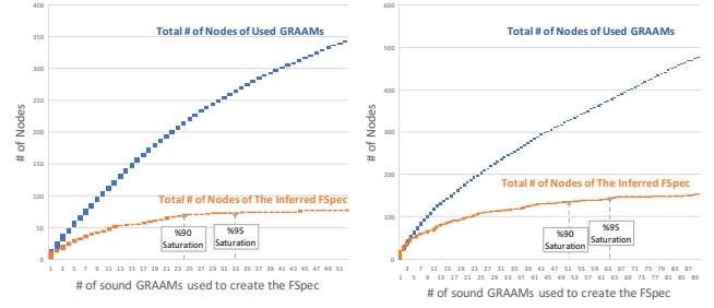
(a) ArCode learning curve while visiting 51 JAAS-based sound GRAAMs
