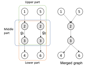
Fig. 7: Emergence of unexpected and unsound sequences by merging g_1 and g_2 from their middle parts
