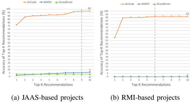
Fig. 11: Accuracy of ARCODE, GrouMiner, and MAPO for fix recommendations on JAAS and RMI experiments
