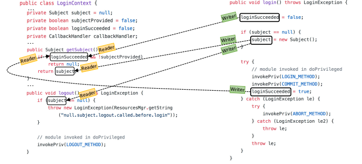
Fig. 3: Extracting Inter-framework Dependencies between g and A
