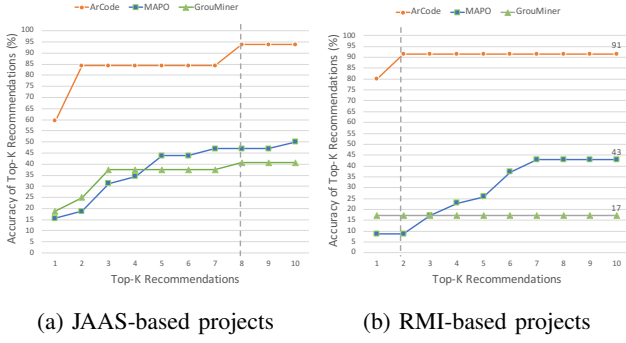
Fig. 9: Accuracy of ARCODE, GrouMiner, and MAPO for next API recommendations on JAAS and RMI experiments
