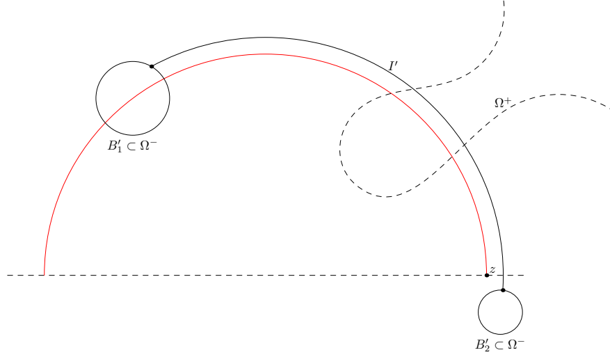
Figure 2. This figure depicts the geometric setup in the proof of Claim 3 . In particular, observe the arc I' with end-points belonging to \Omega^- that intersects \Omega^+ .
