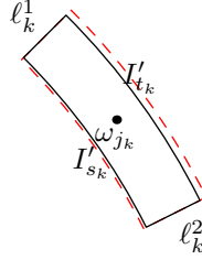
Figure 4. The figure depicts the solid black lined tubular neighborhood \widetilde{U}_k and the red dashed neighborhood U_k .
