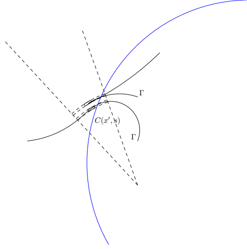
Figure 3. This figure depicts a circumference C(x', s) crossing X_{j_0, k_1} to the right of \tilde{X}_{j_0, k_1} and crossing X_{j_0, k_2} to the right of \tilde{X}_{j_0, k_2} .
