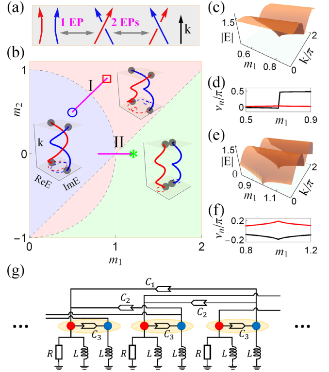
FIG. 2. Phase diagram and phase transitions of H_{12}(k) defined in Eq. (7). (a) Schematic of knot transitions. Type-I (type-II) transition occurs by going through one (two) EP. (b) The phase diagram of H_{12} with parameters m_1 and m_2 . The blue, pink, and green regions label the Hopf link ( \tau_1^2 ), unknot ( \tau_1 ), and unlink phase ( \tau_1^0 ), respectively. In each region, a representative band structure is plotted. (c) and (e) Eigenenergy |E(m_1, k)| along the cut labeled by I and II, respectively, in (b): an EP is visible at (1/\sqrt{2}, \pi) in (c), while there are two EPs at (1, 0) and (1, \pi) in (e). (d) and (f) The Wannier centers \nu_n along the cut I and II. (g) Schematic of a periodic electric circuit that realizes H_{12} . The unit cell (oval) contains two “sites,” the red and blue nodes, connected by resistors R , inductors L , and negative impedance converters C_{1,2,3} ; see Supplemental Material [81] for details.
