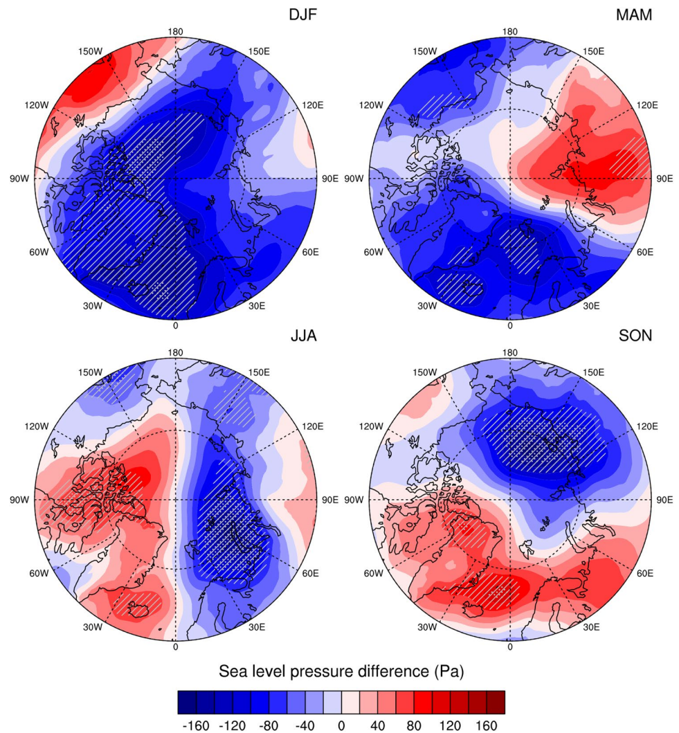
Fig. 5 Difference of sea level pressure between “big kick” ensemble mean and control for each season, defined by the months indicated, for the period 2035–2065, stippled where the difference is significant at the 90% level and hatched where the difference is significant at the 80% level
