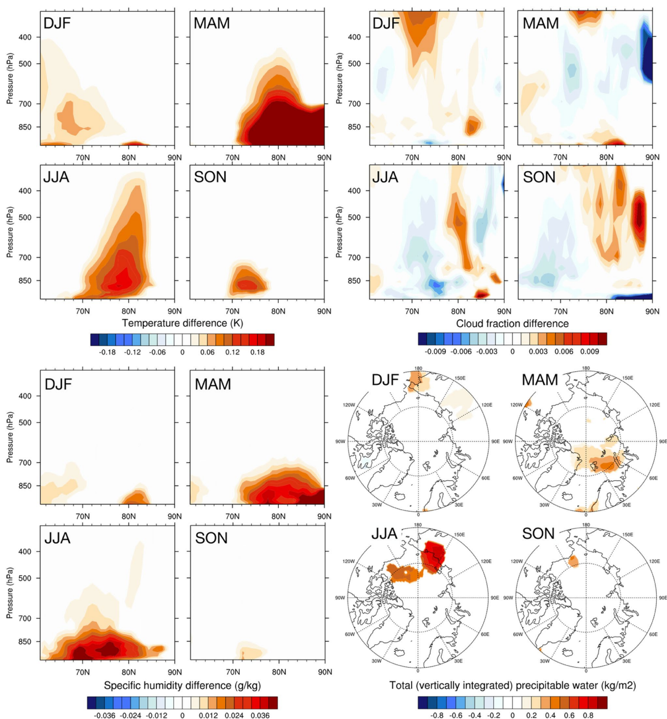
Fig. 4 Seasonal difference in temperature, cloud fraction, specific humidity, and total precipitable water between “big kick” ensemble mean and control from 2035 to 2065. The first three variables
