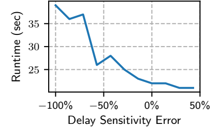
Figure 7: Impact of error in estimating delay sensitivity on MILC runtime
