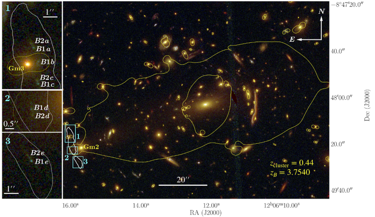
Figure 2. Same as Fig. 1, while highlighting the configuration of System B . The white contours indicate the \text{Ly}\alpha emission associated with System B at \text{SB}_{\text{Ly}\alpha} = 2.8 \times 10^{-18} \text{ erg s}^{-1} \text{ cm}^{-2} \text{ arcsec}^{-2} , integrated over the spectral window of 5766–5796 Å (see Section 5.1 below). The surface brightness limit corresponds to a 3\sigma limiting flux over a circular aperture of 1 arcsec in diameter, roughly the size of the PSF measured in the MUSE data. The yellow contours show the critical curve of the cluster lens for a source at z = 3.754 . The left-hand panels show zoomed-in regions around the lensed images of galaxy B consisting of components B1 and B2 , along with the \text{Ly}\alpha contours. Cluster member galaxies Gm2 and Gm3 are located close to lensed images of System B and are individually optimized in the lens modelling process as described in Section 3. After correcting for the lensing magnification, the total \text{Ly}\alpha luminosity from the nebula is L_{\text{Ly}\alpha} = (9.8 \pm 0.2) \times 10^{41} \text{ erg s}^{-1} (see Section 5.1).
