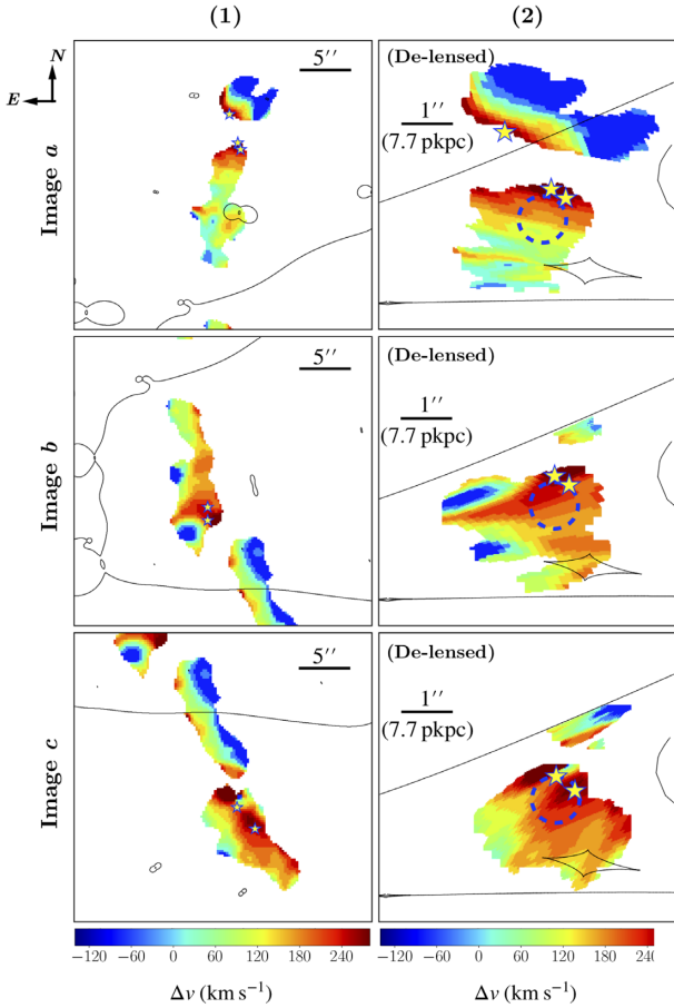
Figure 11. Column (1): velocity map of multiple images a , b , and c in System A, derived from cross-correlating the best-fitting shell model for the template spectrum (bottom-left panel of Fig. 10) and spectra extracted from spaxels within the 3\sigma contours. Zero velocity corresponds to z_{\text{sys}} = 3.0364 , which is the systemic redshift of A1 derived from nebular emission lines. Column (2): de-lensed velocity map of individual images in the source plane. The star symbols mark the positions of the associated star-forming galaxies identified in HST images (see Figs 6 and 7). The blue dashed circles, same as in Column (2) of Fig. 7, mark the apertures for the template spectrum extraction, which we use for the shell model analysis.
