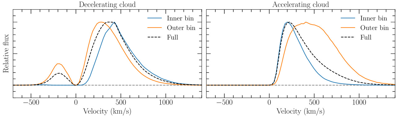
Figure D1. Left-hand panel: Emergent \text{Ly}\alpha profiles extracted from the inner and outer bins of a decelerating expanding cloud. The inner and outer bins correspond to the projected distance range of [0, 0.5R_{\text{max}}] and [0.5R_{\text{max}}, R_{\text{max}}] from the centre of the cloud, respectively, where R_{\text{max}} is the radius of the cloud. The dominant red peak of the \text{Ly}\alpha profiles is more blueshifted in the outer bin. The full spectrum extracted from the entire cloud is shown in the dashed black curve. Right-hand panel: same as the left-hand panel but for an accelerating expanding cloud. The profile is more redshifted in the outer bin, contrary to the trend observed for a decelerating cloud.
