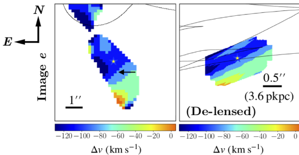
Figure 12. Left-hand panel: velocity map of image e in System B, derived from cross-correlating the best-fitting shell model for the template spectrum (bottom-right panel of Fig. 10) and spectra extracted from spaxels within the 3\sigma contour. Zero velocity corresponds to z_{\text{sys}} = 3.7540 , which is the systemic redshift of B1/B2 derived from nebular emission lines. Right-hand panel: de-lensed velocity map of image e in the source plane. The star symbols mark the position of B1/B2 determined from HST images (see Fig. 8). The black arrow, same as in Column (1) of Fig. 8, indicates the brightest pixel in image e that is included in the template spectrum.
