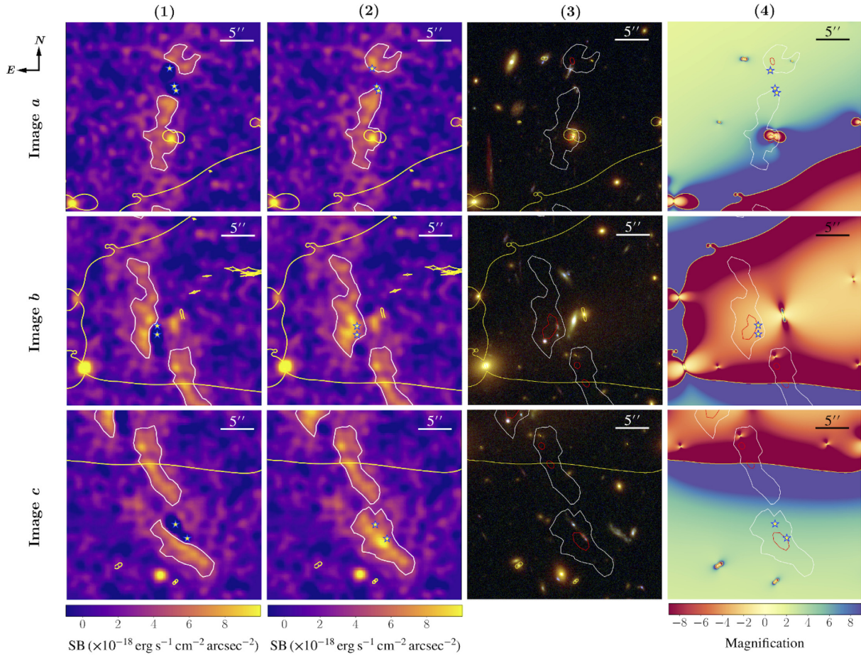
Figure 6. Summary of the lensing configuration of the observed Ly \alpha arc in System A. Column (1): pseudo narrow-band images without the emergent Ly \alpha flux within the DLA troughs at the locations of galaxy continuum. The images have been smoothed using a Gaussian kernel of \text{FWHM}_{\text{smooth}} = 1 arcsec. The contour marks constant surface brightness of 3.7 \times 10^{-18} \text{ erg s}^{-1} \text{ cm}^{-2} \text{ arcsec}^{-2} , which is detected at the 3\sigma level of significance in the smoothed image. The star symbols mark the positions of the associated star-forming galaxies identified in HST images. Column (2): same as Column (1) but includes Ly \alpha flux from the DLA troughs at the locations of galaxy continuum (see text). Column (3): contours of multiply lensed Ly \alpha nebulae determined from Column (2) overlaid on individual galaxy images in the HST data to illustrate the relative alignment between star-forming regions and the line-emitting gas (see also Fig. 1). Ly \alpha surface brightness contours of 3.7 \times 10^{-18} and 7.3 \times 10^{-18} \text{ erg s}^{-1} \text{ cm}^{-2} \text{ arcsec}^{-2} are shown in white and red, respectively, and the yellow contours mark the critical curves of the cluster lens for sources at z = 3.038 . Column (4): the magnification map overlaid with the same Ly \alpha contours to illustrate the spatial variation of lensing magnification across the nebulae. Negative magnification factors indicate flipped parity of the image.
