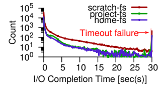
Figure 5: WriEx measured latency on three file partitions.
