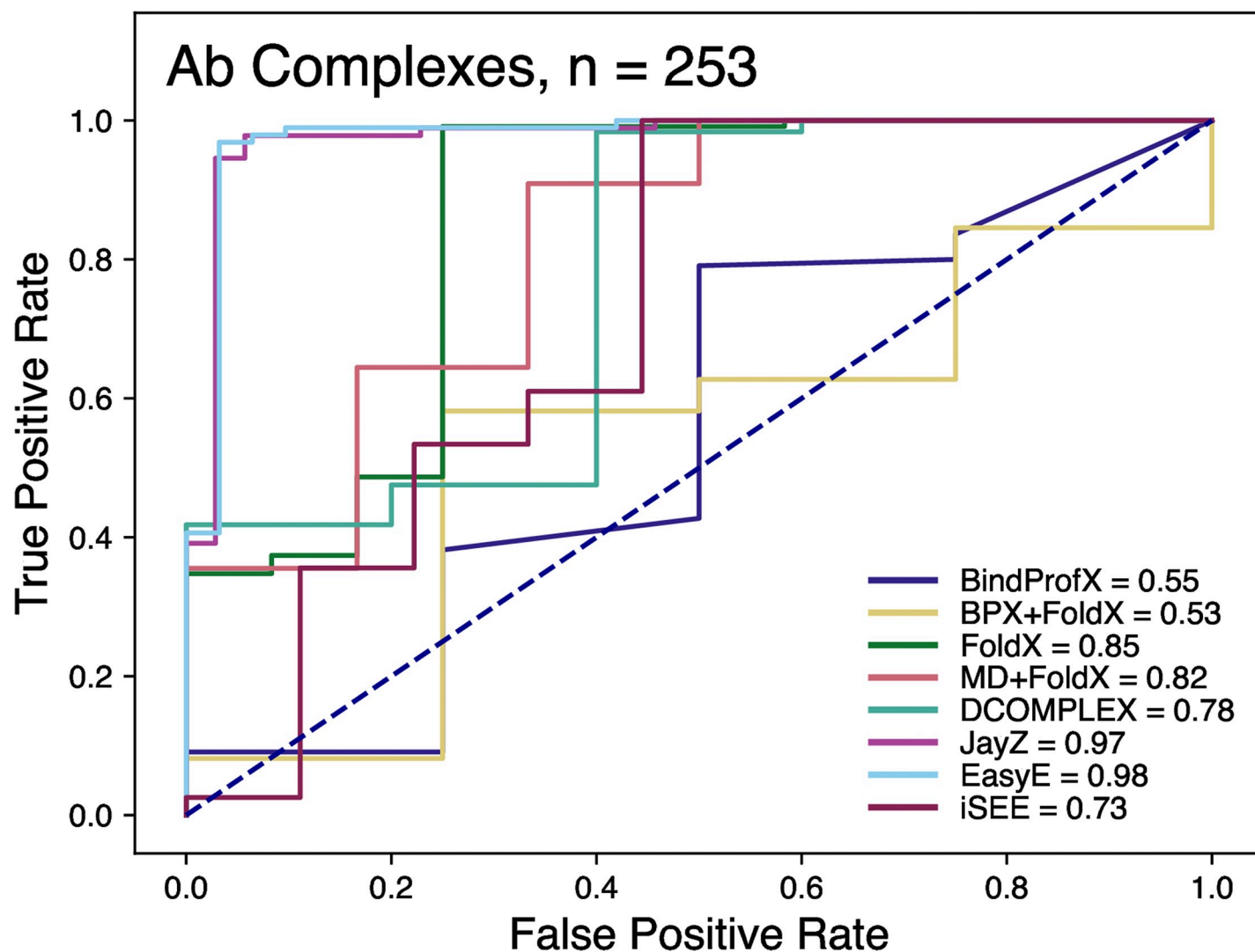
Fig 5. Receiver operating characteristic curves of the classification of variants that are more destabilized or less destabilized than 0.5 kcal/mol. The values in the legend represent the area-under-curve (AUC). The higher the value, the better the prediction capability of the method.
