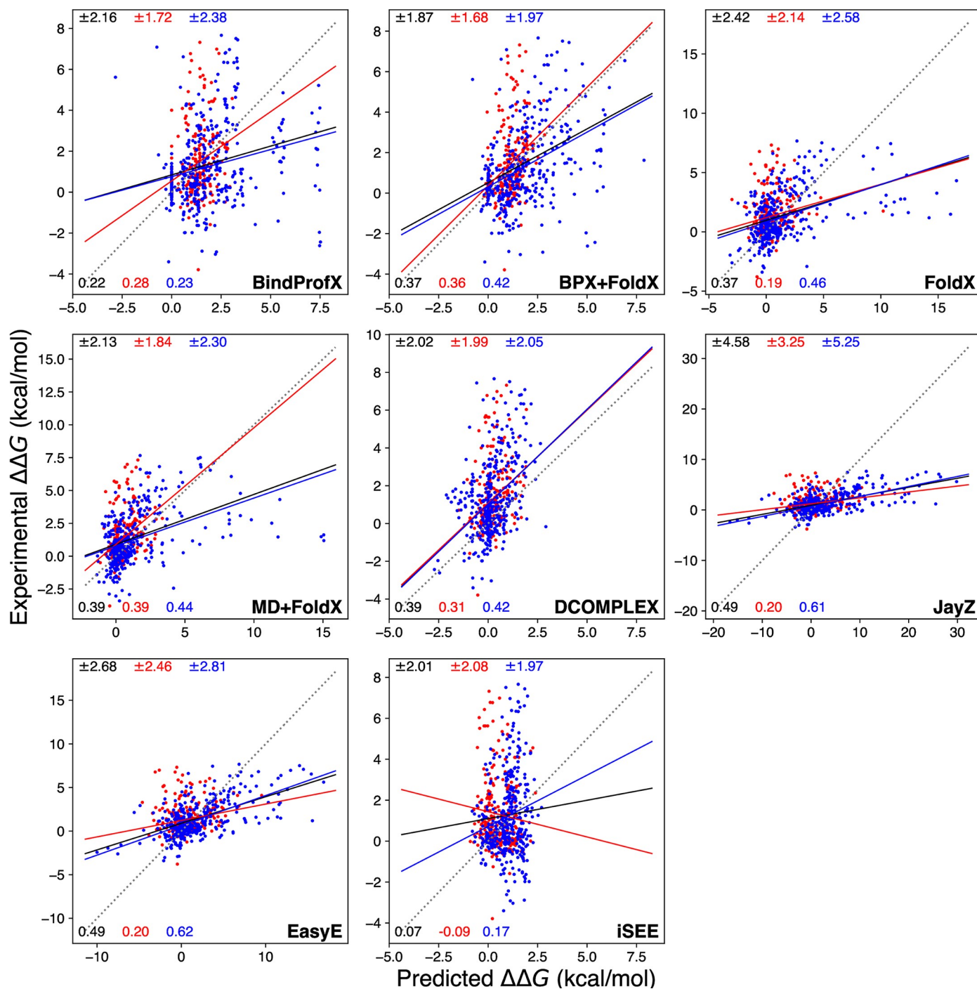
Fig 1. Calculated \Delta\Delta G values (x-axis) compared to experimental \Delta\Delta G values (y-axis) for each method tested in this study. Black, red, and blue lines are simple linear regressions from which r are derived. The red points are a scatter for Ab complexes and the blue points are for non-Ab complexes. The dashed line is the y = x line measuring perfect agreement between predicted and experimental \Delta\Delta G values. The solid black, red, and blue lines indicate a linear relationship between calculated and experimental observations for all data points, Ab complexes, and non-Ab complexes respectively. The top values in black, red, and blue match the root-mean-square error and the bottom values indicate r for all values, Ab values, and non-Ab values respectively.
