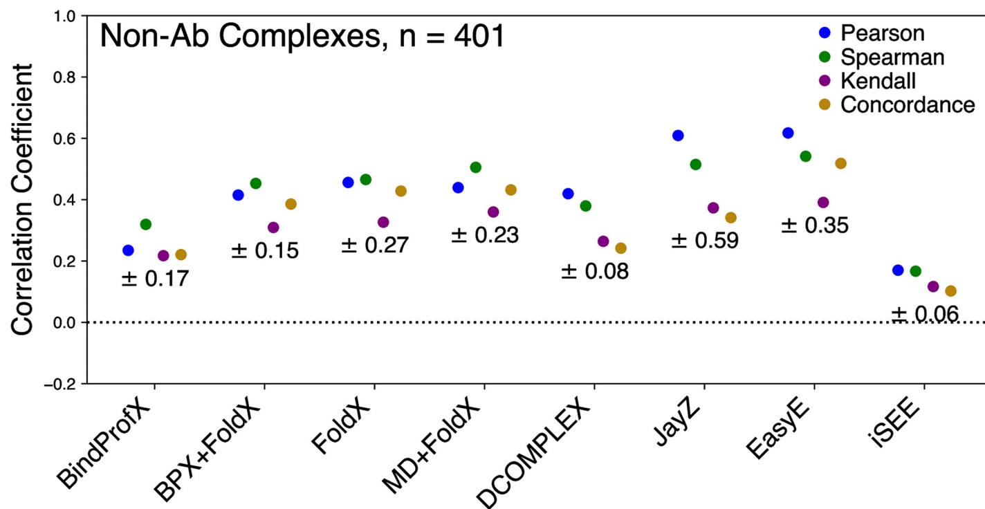
Fig 2. Performance of each method for non-Ab complexes (401 total mutations) in predicting true \Delta\Delta G values ( \rho_c ), linearly correlated \Delta\Delta G values ( r ), and rank order ( \rho and \tau ). The error for each method is reported under the correlation points.
