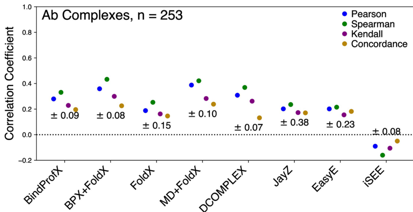
Fig 4. Performance of each evaluated method for Ab complexes (253 total mutations) in predicting true \Delta\Delta G values ( \rho_c ), linearly correlated \Delta\Delta G values ( r ), and rank order ( \rho and \tau ). The error for each method is reported under the correlation points.
