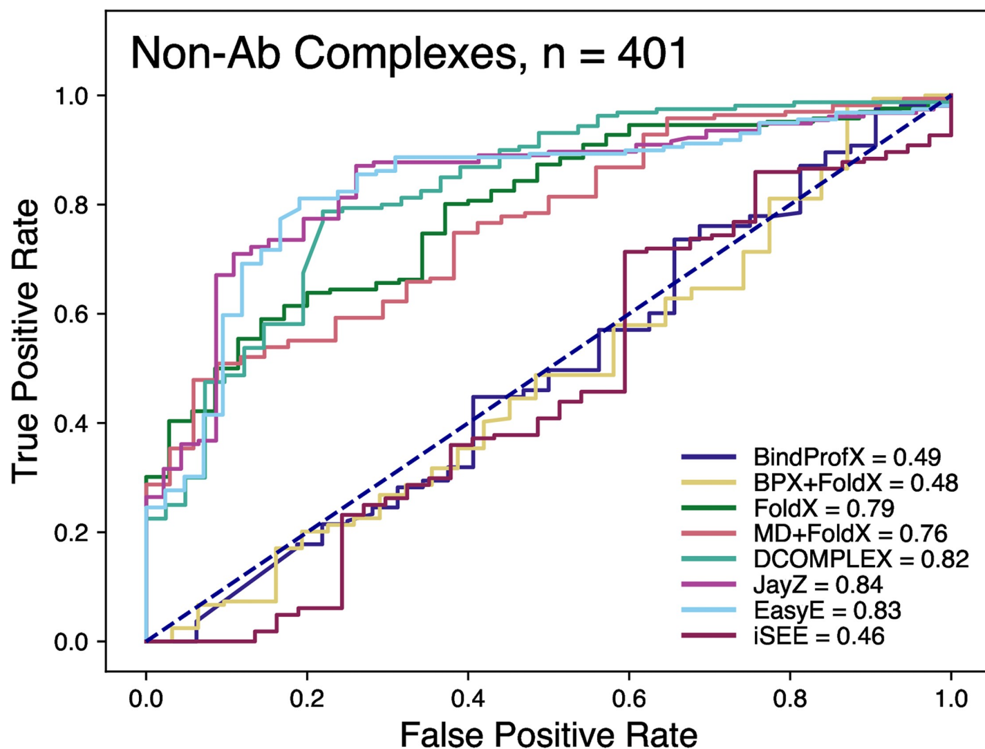
Fig 3. Receiver operating characteristic (ROC) curves for non-Ab complexes of the classification of variants as stabilizing ( \Delta\Delta G < -0.5 kcal/mol) or destabilizing ( \Delta\Delta G > 0.5 kcal/mol). The values in the legend represent the area-under-curve (AUC). The higher the value, the better method is at discriminating between destabilizing and destabilizing mutations.
