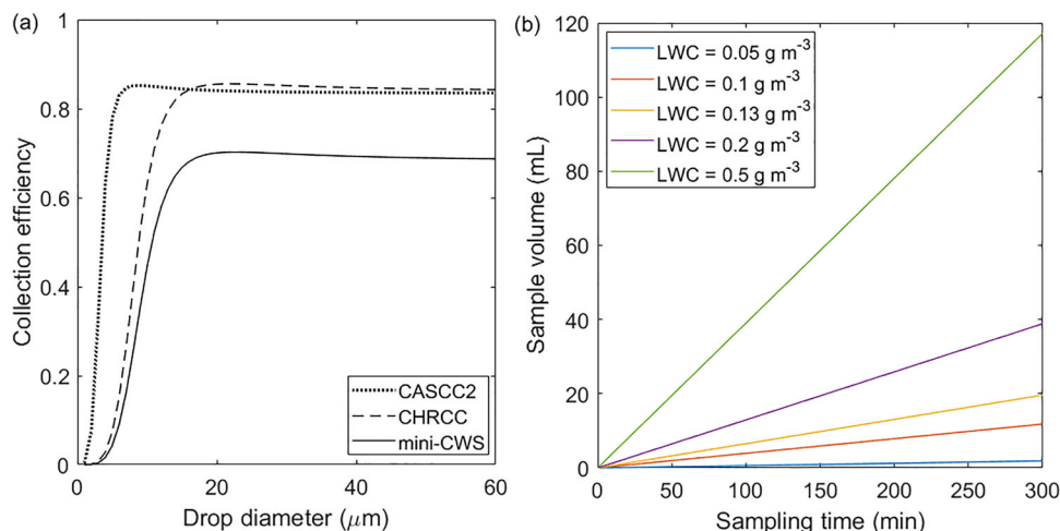
Fig. 3. (a) Theoretical collection efficiency of the mini-CWS compared to the CASCC2 and CHRCC (Demos et al., 1996) based on their respective sampling velocities ( 1.4 \text{ m s}^{-1} for the mini-CWS and 8.6 \text{ m s}^{-1} for the CASCC2 and CHRCC) and (b) estimated sample volume for the mini-CWS for different LWCs.
