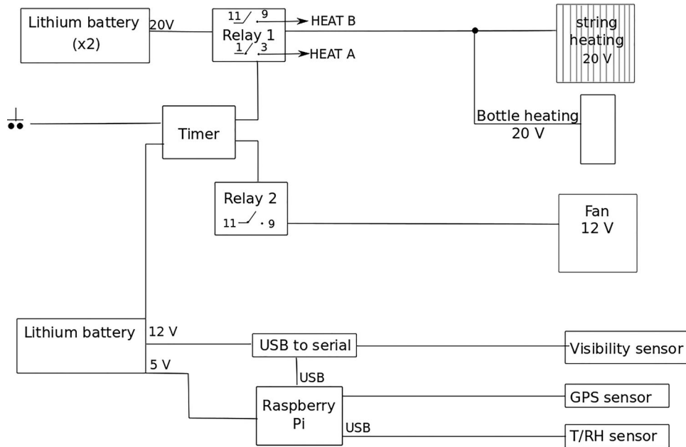
Fig. 2. Schematic circuit diagram of the mini-CWS.
