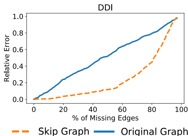
Figure 6. The ability of skip graph and original graph to capture the network structure in the face of incomplete data. Skip graph can better preserve the network structure than the original graph, as evidenced by skip graph's smaller relative error ("Robust learning on incomplete interaction network" section) than that of the original graph. This is true for all % of missing edges, indicating that skip graph can keep useful information about interaction structure even when networks are highly incomplete and many interactions are missing.
