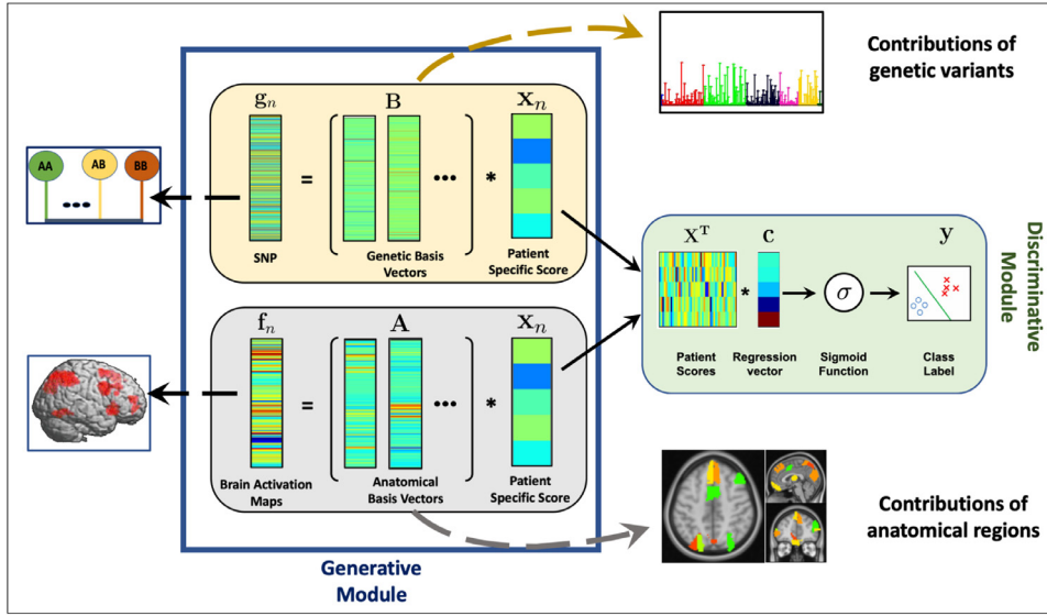
Fig. 1. Generative-discriminative framework linking imaging ( \mathbf{f}_n ), genetics ( \mathbf{g}_n ), and diagnosis ( y_n ). The generative module captures the brain activations and the genetic data in a dictionary learning setup, and the discriminative module tracks the disease status using logistic regression. The classification module also guides the generative process to find a low dimensional space where the patient specific scores \mathbf{x}_n are maximally separated. Therefore, the basis vectors \{\mathbf{A}, \mathbf{B}\} identify biomarkers which capture group level differences between patients and controls. We have shown representative contributions of these basis vectors in the form of a Manhattan plot and a colored brain plot.
