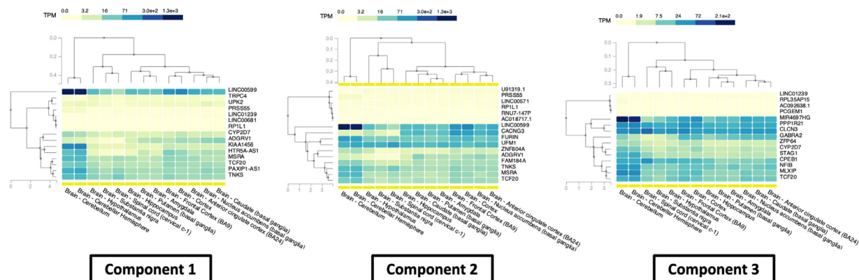
Fig. 11. The gene expression pattern of the top genes identified from the N-Back task based on the GTEx database.
