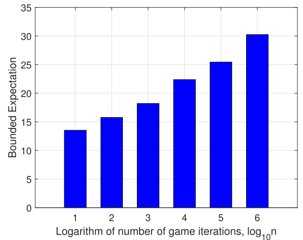
FIGURE 2. BE vs. the logarithm of the number of St. Petersburg game iterations, assuming \epsilon = 10^{-3} .
