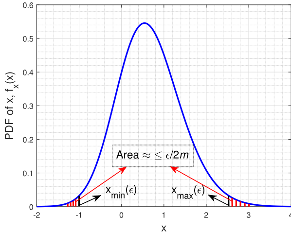
FIGURE 1. The values of x_{\min}(\epsilon) and x_{\max}(\epsilon) for a random variable with PDF f_X(x) .
