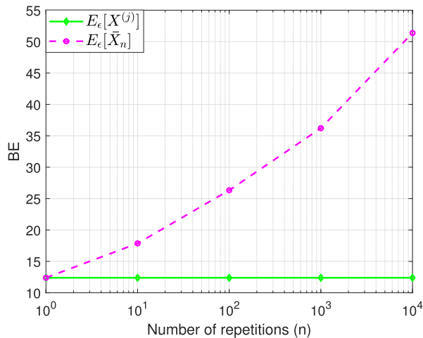
FIGURE 3. BE of the sample mean of the right-tailed Pareto random variables, E_{\epsilon}[\bar{X}_n] , and the BE of X^{(j)} s vs. the number of repetitions n for the case of infinite expected value, assuming \epsilon = 0.001 .
