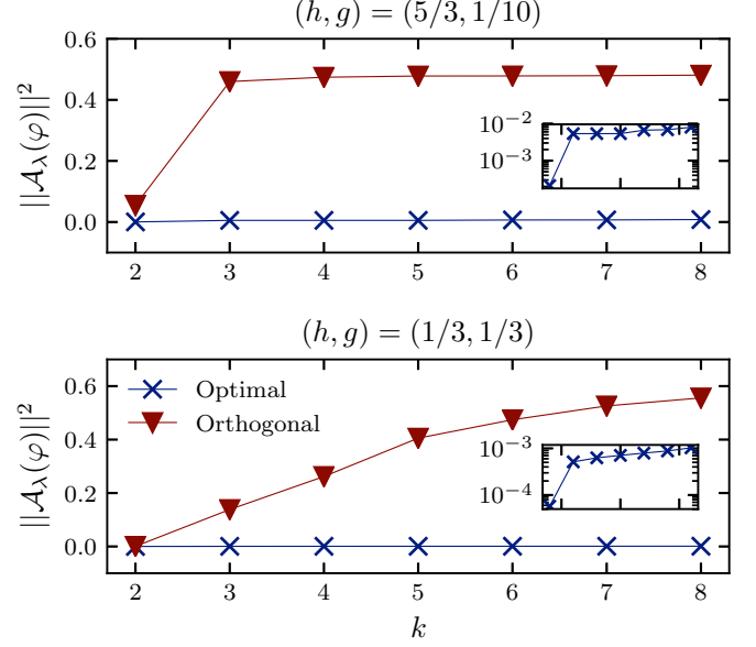
FIG. 8. The norm of the VAGP for different ansatz sizes k . The upper figure corresponds to (h, g) = (5/3, 1/10) and the lower figure to (1/3, 1/3) . The blue (red) points are the norms of the VAGP in the optimal (orthogonal) direction. The VAGP shows a high degree of anisotropy for k \gtrsim 3 . (Inset) Semilogarithmic plot of the norm of the VAGP in the optimal direction. It is consistent with exponential growth of the norm as a function of k , but the exponent is extremely small.
