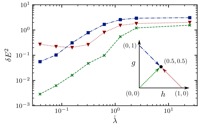
FIG. 3. Final energy variance of a generic initial eigenstate as function of protocol rate for unassisted adiabatic state preparation. The end point is given by (0.5, 0.5) and initial points are given by (\epsilon, \epsilon) (optimal), (1 - \epsilon, \epsilon) and (\epsilon, 1 - \epsilon) (both orthogonal) with \epsilon = 10^{-2} , as shown in the inset. System size is L = 12 . The optimal path always outperforms the orthogonal ones.
