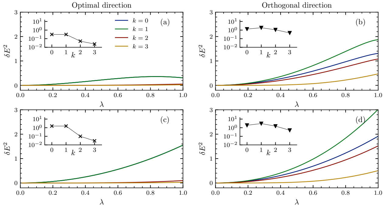
FIG. 4. Energy variance of a generic initial eigenstate evolved along the optimal direction with finite \dot{\lambda} [top row (a, b)] and with infinite \dot{\lambda} [bottom row (c, d)] along either the optimal direction [left column (a, c)] or the orthogonal one [right column (b, d)]. Full lines show the energy variance during the protocol as function of \lambda(t) , where the blue lines represent the unassisted protocol ( k = 0 ) and the other lines represent CD driving with k -body VAGPs (12). Since one-body VAGP is exactly zero along the optimal direction, the lines for k = 0 and 1 completely overlap each other. The inset details the energy variance at the end of the protocol as a function of k . The end points for both protocols are given by (h, g) = (0.5, 0.5) , with the optimal protocol starting from (\epsilon, \epsilon) and the orthogonal one from (1 - \epsilon, \epsilon) (see also inset of Fig. 3). System size is L = 12 . In the unassisted protocol, the energy variance is already much smaller along the optimal directions than along the orthogonal directions. Applying local two-body CD driving, the energy variance drastically reduces even more along the optimal direction, while it only gradually decreases in the orthogonal direction. At infinite \dot{\lambda} the state along the optimal direction can similarly be accurately approximated by a two-body dressing of the initial state, whereas the accuracy along the orthogonal direction only gradually increases.
