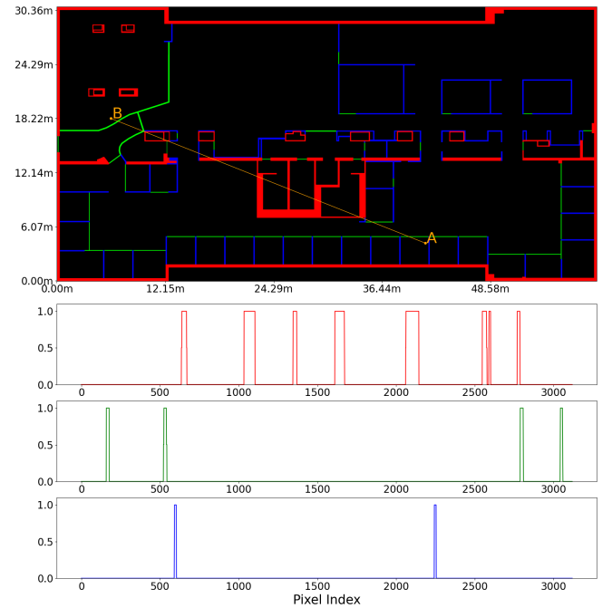
Figure 5: Example ray-trace with its corresponding waveform from A to B
