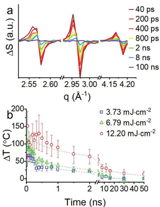
Fig. 4 Transient X-ray diffraction patterns of 50 nm TiN NPs excited at a 400 nm pump fluence of 6.79 \text{ mJ cm}^{-2} for the indicated pump–probe delay times ranging from 40 ps to 100 ns. (b) Estimated temperature changes of 50 nm TiN NPs versus time for stated fluences of 400 nm pump excitation. Temperatures are estimated as described in the text with errors bars representing high and low estimates from (111), (200), and (220) peaks. Dashed gray lines show stretched exponential fits to the data.
