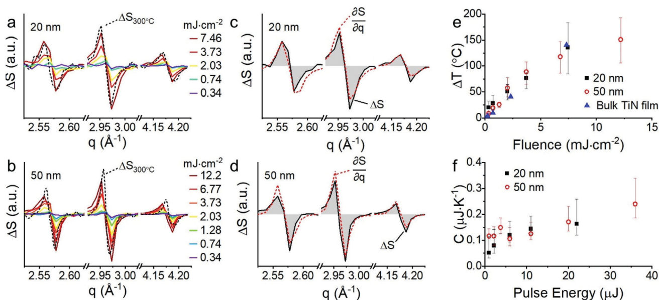
Fig. 3 (a and b) Selected transient X-ray diffraction data ( \Delta S ) for (a) 20 nm and (b) 50 nm TiN NPs for several fluences specified in the legends. All displayed data were collected at 40 ps pump-probe delay using 400 nm pump excitation. Overlaid on the transient X-ray diffraction data are dashed lines showing thermal difference diffraction curves, \Delta S_{300^\circ\text{C}} , based upon temperature-dependent powder diffraction patterns at 300 °C and 25 °C. \Delta S_{300^\circ\text{C}} curves were multiplied to overlay transient X-ray diffraction data. (c and d) Selected transient X-ray diffraction data for (c) 20 nm and (d) 50 nm TiN NPs, shown with black lines. Gray shading indicate the area under the peak of \Delta S . Data was acquired 40 ps after photoexcitation with 400 nm light at a fluence of 7.46 \text{ mJ cm}^{-2} for 20 nm NPs and 12.20 \text{ mJ cm}^{-2} for 50 nm NPs. The dashed red curve is the first derivative of the static scattering data before pump excitation, multiplied by \Delta q of -0.0011 \text{ \AA}^{-1} for (c) and -0.0014 \text{ \AA}^{-1} for (d). (e) Estimated lattice temperature change at 40 ps pump-probe delay for the 20 nm and 50 nm TiN NP samples against 400 nm excitation fluence. Estimates are calculated by averaging data from the (111), (200), and (220) reflections with error bars spanning the highest and lowest estimated values. Also shown on the plot is the change in lattice temperature reported for 400 nm excitation of bulk TiN films using transient thermoreflectance. 36 (f) Heat capacity of samples as a function of pulse energy. Estimates of heat capacity are calculated by using average, high, and low estimates of temperature change.
