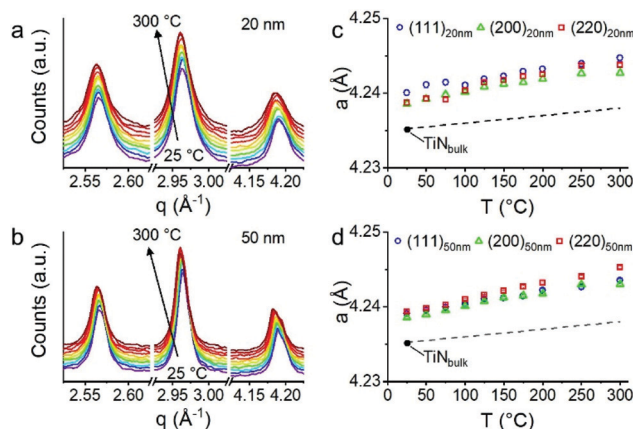
Fig. 2 (a and b) Representative static powder X-ray diffraction of (a) 20 nm and (b) 50 nm TiN NPs as a function of temperature from 25 °C to 300 °C. Data are shown in a rainbow scale from low temperature (violet) to high temperature (red). Data are offset vertically for clarity. (c and d) Cubic lattice parameter estimates based upon fitted values of the (111), (200), and (220) reflections for (c) 20 nm and (d) 50 nm TiN NPs. Dashed lines in (c and d) indicate the bulk thermal expansion of TiN. 52
