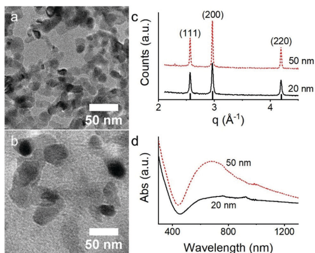
Fig. 1 (a and b) Transmission electron microscopy images of (a) 20 nm TiN NPs and (b) 50 nm TiN NPs. (c) Powder X-ray diffraction of 20 nm and 50 nm TiN NPs. Cubic reflections of bulk TiN are shown in black lines. 50 (d) Visible absorption spectra of 20 nm and 50 nm TiN NPs.
