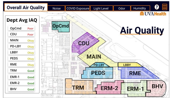
Fig. 2. Figma design
