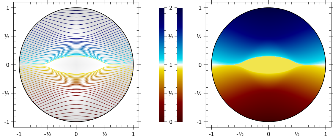
Figure 12: Level sets \partial E_t for t \in (0, 2) in Example 6.9, when the solution is constructed using minimal weak solution sets as the “superlevel pancakes”. Heightmap of u is on the right; the color at each point represents the solution’s value there.
