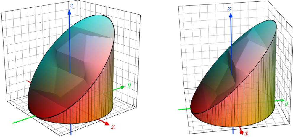
Figure 7: Graph of the solution u of the Dirichlet problem in Example 6.5, depicted as a surface z = u(x, y) .
