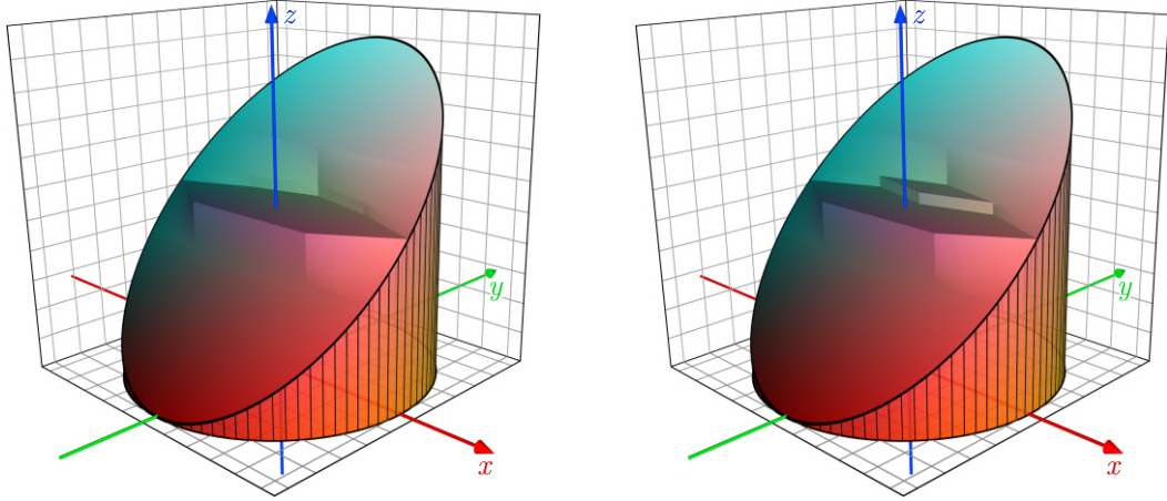
Figure 11: Graphs of the two distinct solutions in Example 6.8 whose level sets have been depicted in Figure 10.
