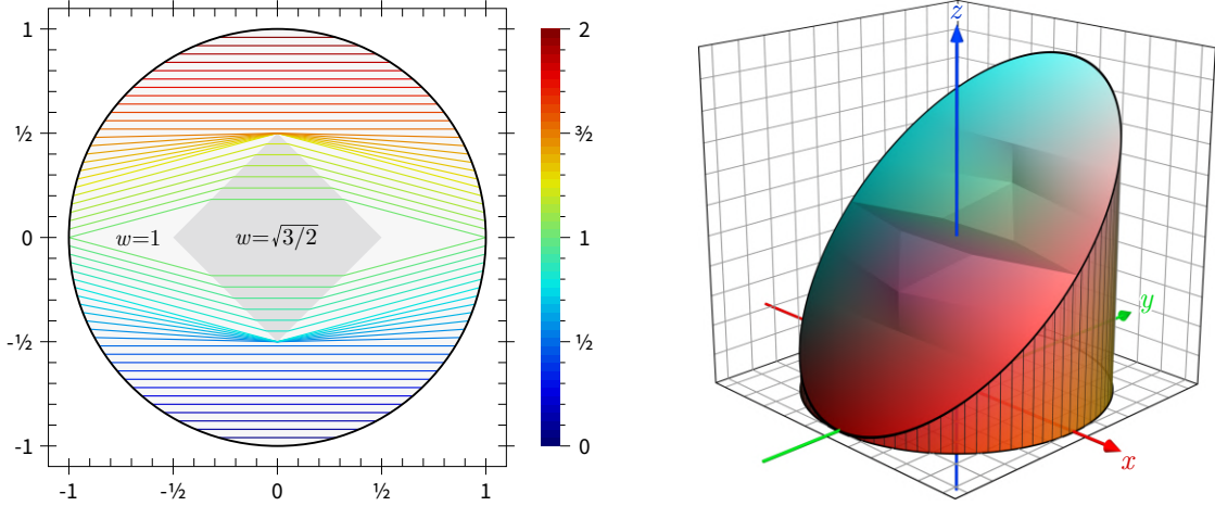
Figure 4: Level sets \partial E_t for t \in (0, 2) in Example 6.3 (b), with \alpha = \sqrt{3/2} , are on the left. Graph of u is on the right. Displacement of level sets from center depends on \alpha .
