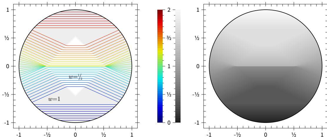
Figure 6: Level sets \partial E_t for values of t \in (0, 2) in Example 6.5, with \alpha = 1/2 , are on the left. A heightmap of the solution u constructed by stacking the sets E_t is on the right, where the grayscale intensity represents the solution's function value.
