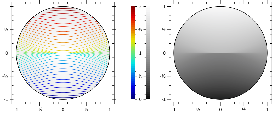
Figure 8: Level sets \partial E_t for various values of t \in (0, 2) in Example 6.6, with \alpha = 1/2 , are shown on the left. A heightmap of the solution u constructed by stacking the sets E_t is shown on the right.
