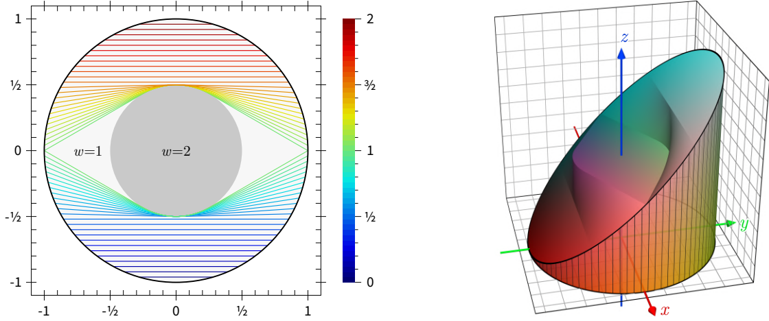
Figure 5: Level sets \partial E_t for various values of t \in (0, 2) in Example 6.4, with \alpha = 2 > \pi/2 , are shown on the left. A graph of the solution u constructed by stacking the sets E_t is shown on the right.
