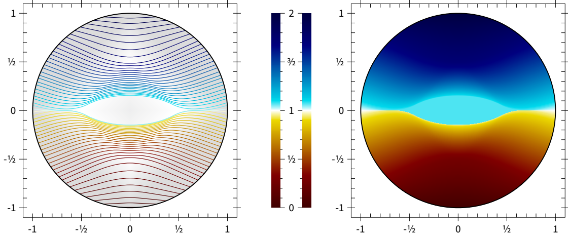
Figure 13: Level sets and a heightmap of the solution in Example 6.9 constructed using maximal weak solution sets as the “superlevel pancakes”. Note that u(x, y) = 2 - \tilde{u}(x, -y) , where \tilde{u} is the solution shown in Figure 12.
