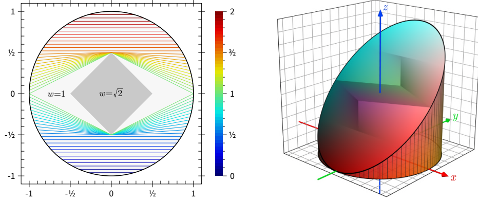
Figure 3: Level sets \partial E_t for t \in (0, 2) in Example 6.3 (a) are shown on the left. Graph of u is shown on the right.
