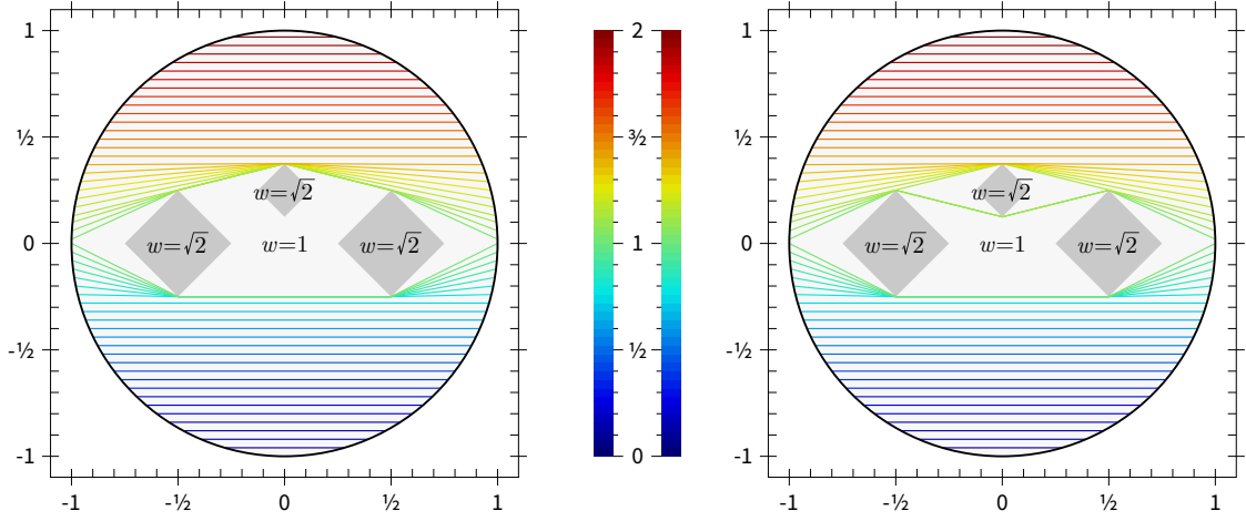
Figure 10: Level sets \partial E_t for various values of t \in (0, 2) in Example 6.8. In the left figure, the shortest path for t_0 < t \leq t_1 passes through the upper tip of the small diamond, and passes through the lower tip in the right figure. Similarly as in Example 6.3 (a), the precise value of \alpha \geq \sqrt{2} plays no role.
