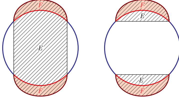
Figure 1: Two weak solutions \chi_E to the Dirichlet problem in \Omega with boundary data \chi_F , where F is the (closed) region filled with light red color. The figure on the right shows the minimal weak solution. Each of the arcs of \partial\Omega \cap \partial F and \partial\Omega \setminus \partial F covers the angle of \pi/2 . Note also that the restriction \chi_E|_{\Omega} is a solution / the minimal solution.
