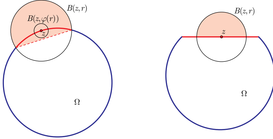
Figure 2: The (Euclidean) domain on the left has boundary of positive mean curvature, unlike the domain on the right. The regions shaded light red in color are weak solution sets of the respective Dirichlet problems.
