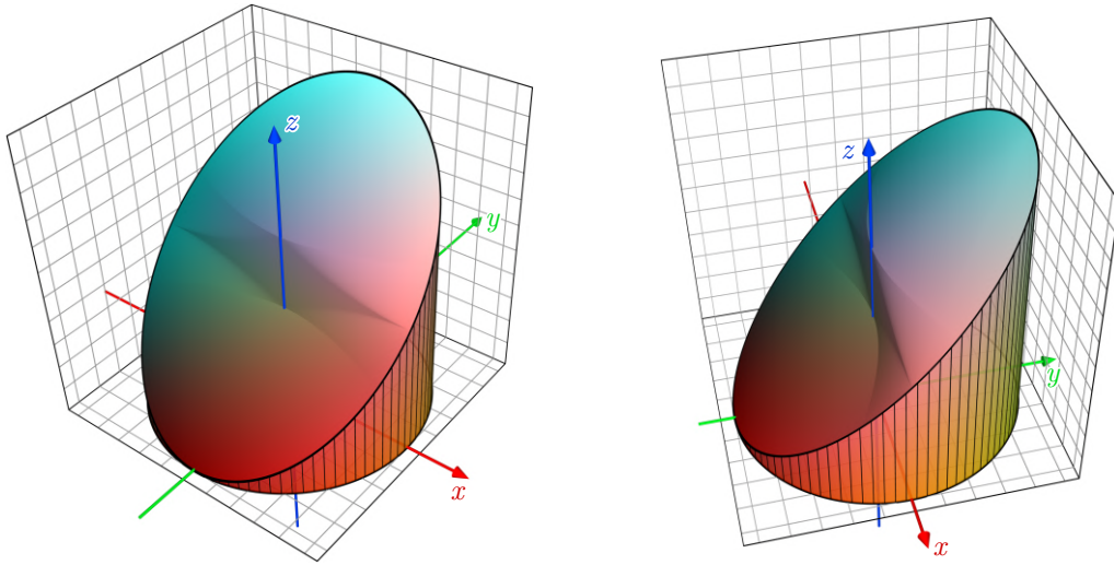
Figure 9: Graph of the solution u of the Dirichlet problem in Example 6.6, depicted as a surface z = u(x, y) . Observe that the jump-set of the solution lies upon the x -axis, i.e., S_u = \{(x, y) \in \Omega : y = 0\} .
