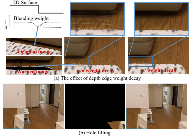
Fig. 9. (a) We decay the weights near occlusion edges to improve the smoothness of view blending. (b) We leverage tile-based rendering [Hedman et al. 2016] to render the pixels inside a hole, and also blend the rendering result with the remaining view warping result with weight decay at the hole boundary.
