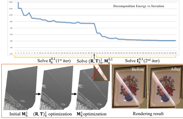
Fig. 11. Convergence curve of the alternating optimization algorithm for reflection decomposition. The rendering results before and after optimization are shown in the last two images in the second row.
