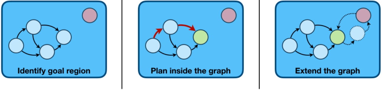
Figure 2. Given a goal (red) outside the graph, the agent uses the graph to plan to reach the node closest to that goal (green). It then expands the graph by constructing a skill chain connecting the goal to the graph.
