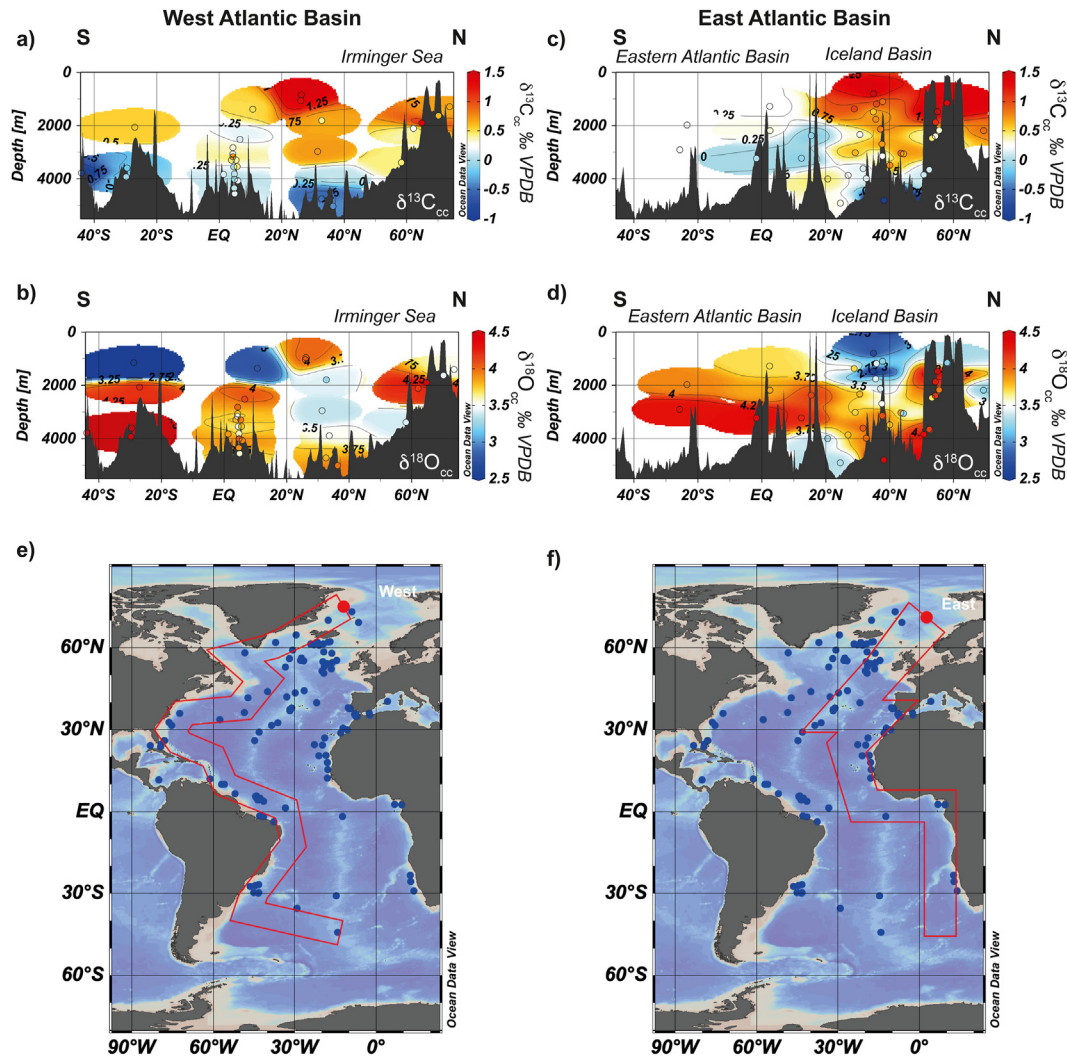
Fig. 2. \delta^{13}\text{C}_{\text{cc}} (a, c) and \delta^{18}\text{O}_{\text{cc}} (b, d) sections across the western (a, b) and eastern (c, d) Atlantic for HS1. Panels (e) and (f) show maps indicating the core locations used for both sections.
