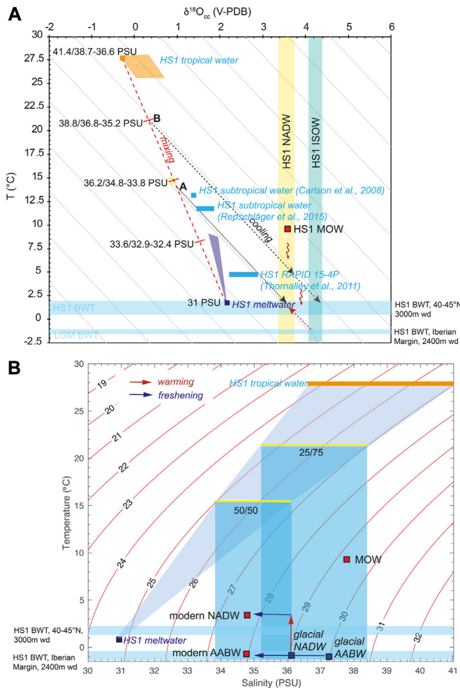
Fig. 8. Mixing of meltwater and subtropical waters as source of the observed deep-water \delta^{18}\text{O}_{\text{cc}} signature during HS1. (a) \delta^{18}\text{O}_{\text{cc}} plotted versus water temperature, with the light-yellow vertical shading indicating the observed range of deepwater \delta^{18}\text{O}_{\text{cc}} data in the deep western Atlantic Basin (NADW) (20–50°N at 1000–4000 m water depth) from this study. The turquoise field indicates \delta^{18}\text{O}_{\text{cc}} data in the Iceland Basin (ISOW) (1000–3000 m water depth) from this study. Grey lines indicate \delta^{18}\text{O}_{\text{cc}} fractionation lines calculated using the equation of Shackleton (1974). The orange field represents the range for tropical surface waters reported by Carlson et al. (2008) and Schmidt and Lynch-Stieglitz (2011). The violet field indicates surface values reported from the subpolar North Atlantic (e.g., Thornalley et al., 2010; Benway et al., 2010), and the dark blue square indicates the HS1 meltwater signature from the inner Labrador Sea (Gibb et al., 2014). (b) Isolines of potential densities (sigma-theta; orange lines) of different mixtures shown on a T-S diagram. Yellow bars correspond to the crossing point of the cooling lines A and B with the water mass mixing line in plot. Red squares indicate modern NADW, AABW (Adkins et al., 2002) and MOW (Locarnini et al., 2013) signatures. Blue squares indicate HS1 meltwater signature (Gibb et al., 2014), and reconstructed glacial deepwater signatures (Adkins et al., 2002). The orange bar represents the reconstructed T-S range of tropical waters (Schmidt and Lynch-Stieglitz (2011)). The horizontal light blue bars in both plots indicate HS1 Bottom Water Temperature (BWT) range reconstructed by Repschläger et al. (2015a) and Skinner and Shackleton (2006), respectively.
