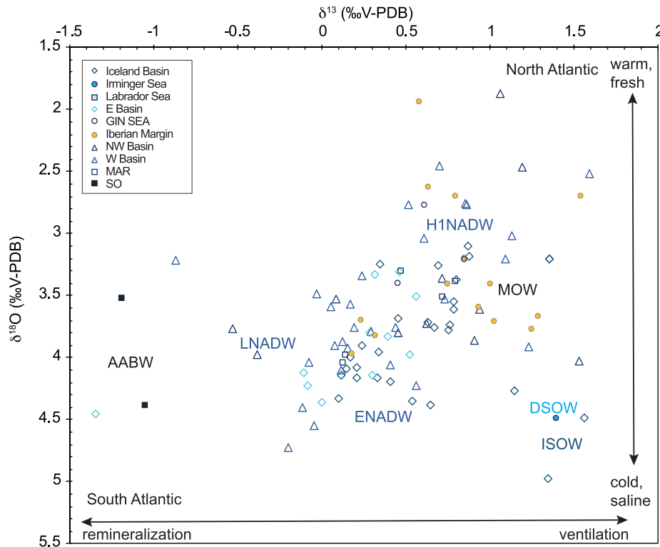
Fig. 5. \delta^{18}\text{O}_{\text{cc}} versus \delta^{13}\text{O}_{\text{cc}} cross plots for the dataset for HS1.
