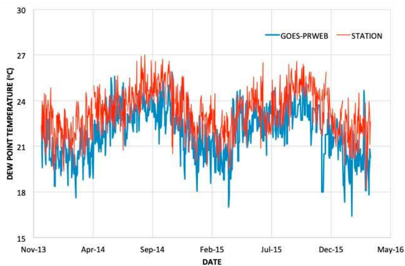
Figure A3. Modeled and observed T_d from January 2014 to April 2016 at the UPR Agricultural Experimental Station near Juan Diaz, Puerto Rico.
