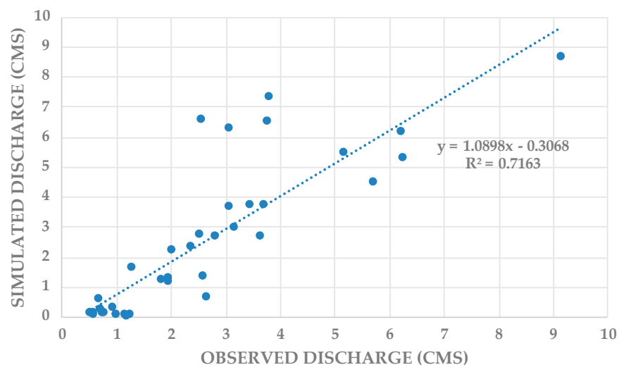
Figure 10. Simulated versus observed stream discharge in the Guanajibo Watershed: observed vs. GOES-PRWEB-estimated RO + DP.
