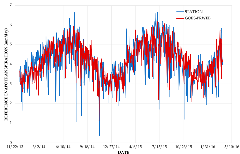
Figure 2. Modeled and observed daily ET_0 from January 2014 to April 2016 at the UPR Agricultural Experimental Station near Juan Diaz, Puerto Rico.
