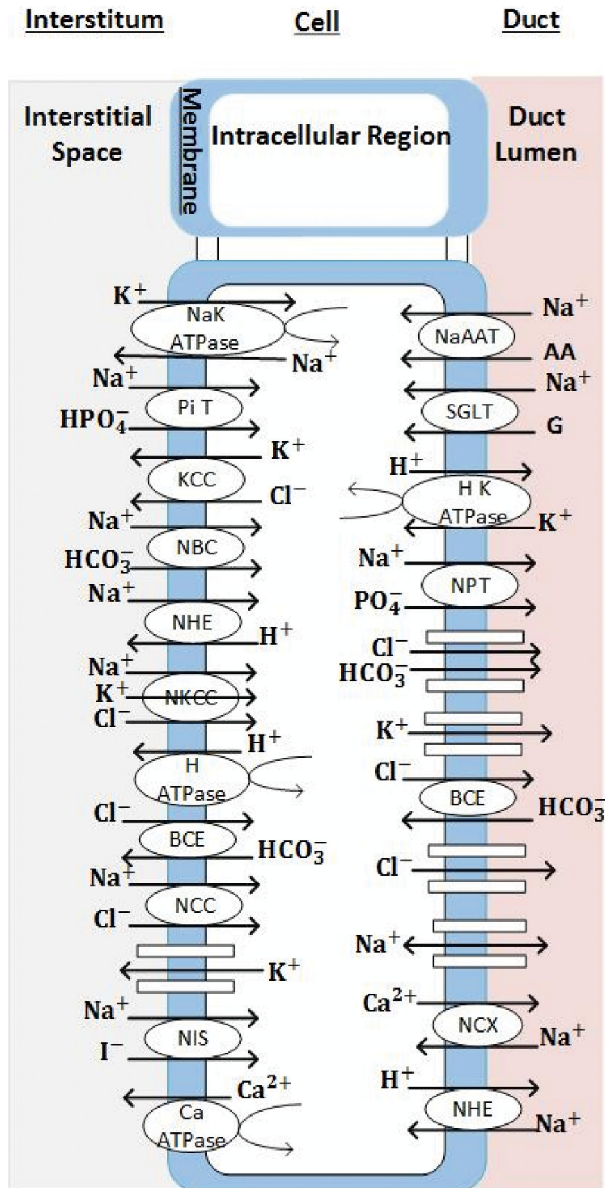
Fig. 1. Schematic representation of most of the important transporters and channels across the cell membrane considered in this work.
