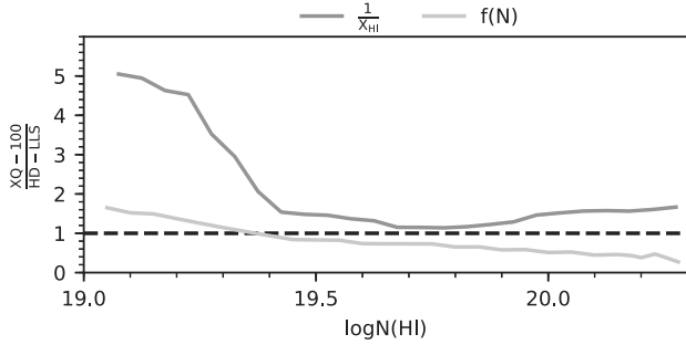
Figure 8. The fractional difference of the assumed neutral fraction ( \frac{1}{X_{\text{HI}}} , dark grey line) and f(N) (light grey line) of this work relative to Fumagalli et al. (2016, \frac{X_{\text{Q-100}}}{X_{\text{HD-LLS}}} ) as a function of \log N(\text{H I}) . Values of \frac{X_{\text{Q-100}}}{X_{\text{HD-LLS}}} > 1 (i.e. above the dashed black line) imply the measured quantity from the method used in this paper is larger than that from Fumagalli et al. (2016). While f(N) has a small difference between the two methods, the neutral fraction can vary by up to a factor of 5 for low column density subDLAs ( \log N(\text{H I}) \lesssim 19.4 ).
