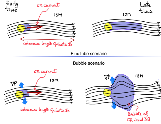
Figure 1: Sketch depicting the main difference between the flux tube scenario and the bubble escape scenario.
