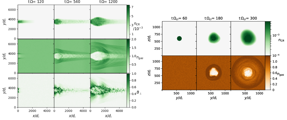
Figure 2: Left panel: CR density and background gas density and magnetic field of the 2D simulation in the xy-plane at three different times. Right panel: CR density and background gas density of the 3D simulation in the yz-plane averaged along the x-axis at three different times.
