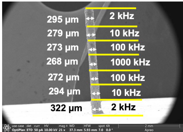
Fig. 6. SEM image of a nickel pillar manufactured at varying pulse frequency conditions.
