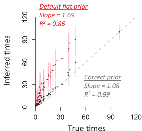
Fig. 2. Comparison of true times with node ages inferred using the correct (black) and the default flat (red) tree prior for the dataset simulated using model tree in Figure 1C. The slope and coefficient of determination ( R^2 ) for the linear regression through the origin are shown. Dots are point estimates of node ages and lines are highest posterior density intervals (HPDs). Gray dashed line is 1:1 line
