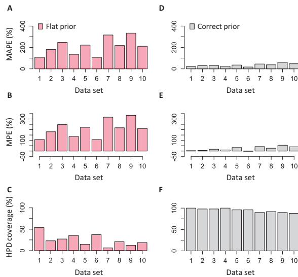
Fig. 5. (A, D) Mean of absolute percent error, MAPE, (B, E) mean of percent error, MPE and (C, F) HPD coverage for nodes times estimated using the default flat (red) and correct (gray) tree prior for each simulated dataset
