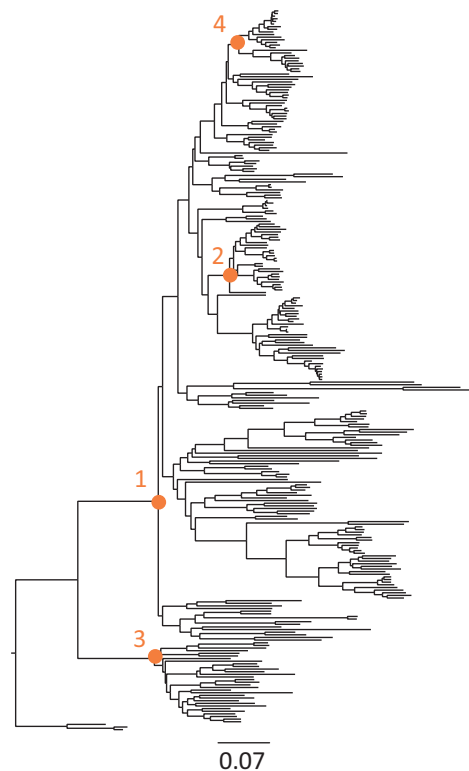
Fig. 3. Evolutionary relationships and branch lengths derived from an alignment of 7370 base pairs of 12 mitochondrial genes from 274 mammalian species from dos Reis et al. (2012). Orange nodes were calibrated in the evaluations in which fewer calibrations were utilized. The number indicates the order of calibration addition
