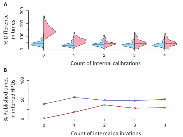
Fig. 11. Analysis of empirical data using different numbers of diffused internal calibrations. (A) Distribution of absolute percent differences between published times and times estimated using ddBD (blue) and the flat (red) tree prior when different numbers of internal calibrations are used. Lines in violin plots are median values. (B) Percent nodes whose published times within HPDs obtained using ddBD (blue) and the flat (red) tree prior when different numbers of internal calibrations are used. Zero on x-axis represents the case where only the root calibration and no internal calibrations are used
