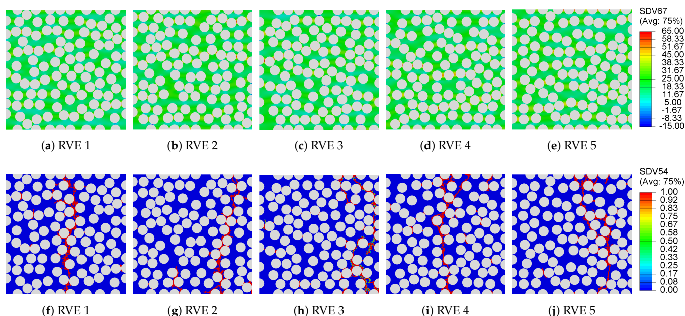
Figure 12. Contour plots of (a–e) maximum principal stresses before the onset of damage and (f–j) damage field in the RVE at the end of the transverse mechanical loading analysis.
