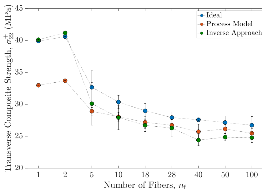
Figure 13. Summary of results from the size effect study showing the transverse composite strength \sigma_{22}^+ as a function of the RVE size n_f for the three material definitions considered.
