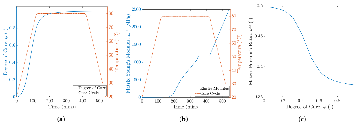
Figure 3. Thermo-mechanical property inputs for RIMR R135/H1366: (a) evolution of the degree of cure with temperature and time, (b) matrix Young's modulus E^m , and (c) matrix Poisson's ratio \nu^m .
