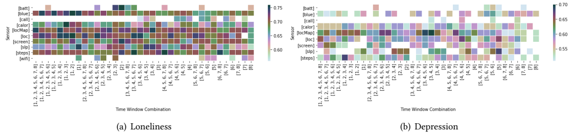
Fig. 7. The heatmap displays the largest F1 score in the loneliness and depression prediction model trained by a combination of different single sensor features and time windows.
