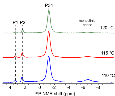
Figure 2. Variable-temperature ^1\text{H} -decoupled ^{31}\text{P} NMR spectra collected between 110 and 120 °C. Peaks p1 and p2 are attributed to the polycations about P1 and P2, respectively, whereas peak p34 is attributed to the polyanions about P3 and P4.
