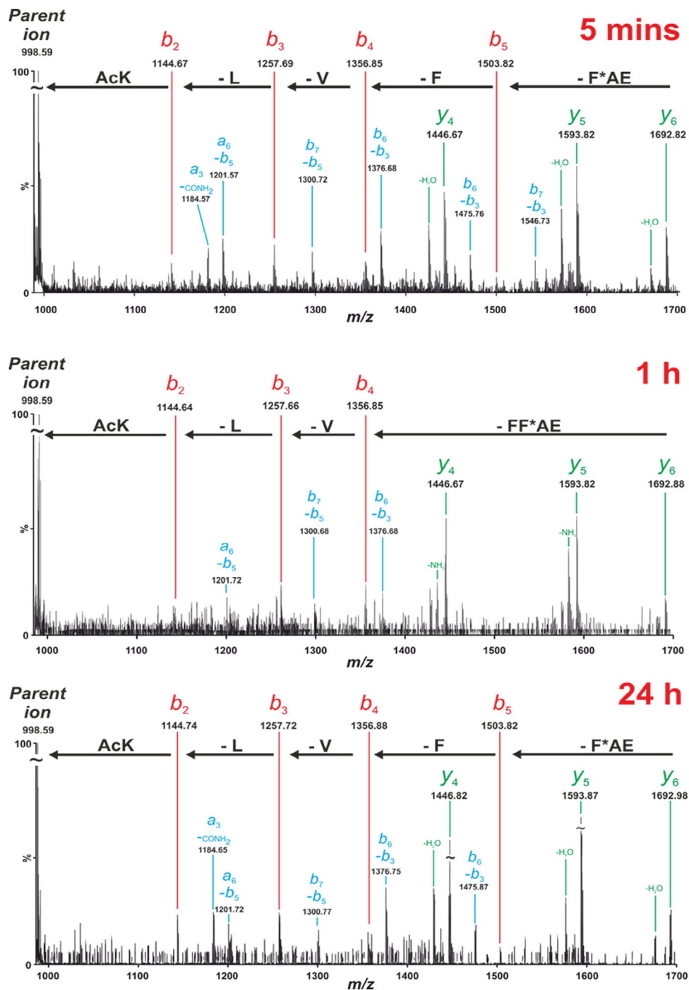
FIGURE 5 Annotated tandem MS/MS spectra demonstrating that at all time points analyzed A \beta^* 16-22 forms anti-parallel, in-register \beta -strands. In the spectra, b ions are highlighted in red, y ions in green and any double fragmentation products in blue [Color figure can be viewed at wileyonlinelibrary.com ]
