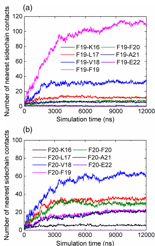
FIGURE 8 Analysis of the closest interpeptide sidechain contacts formed by F19 (a) and F20 (b) with the other residues of A \beta_{16-22} in the system as a function of simulation time [Color figure can be viewed at wileyonlinelibrary.com ]
