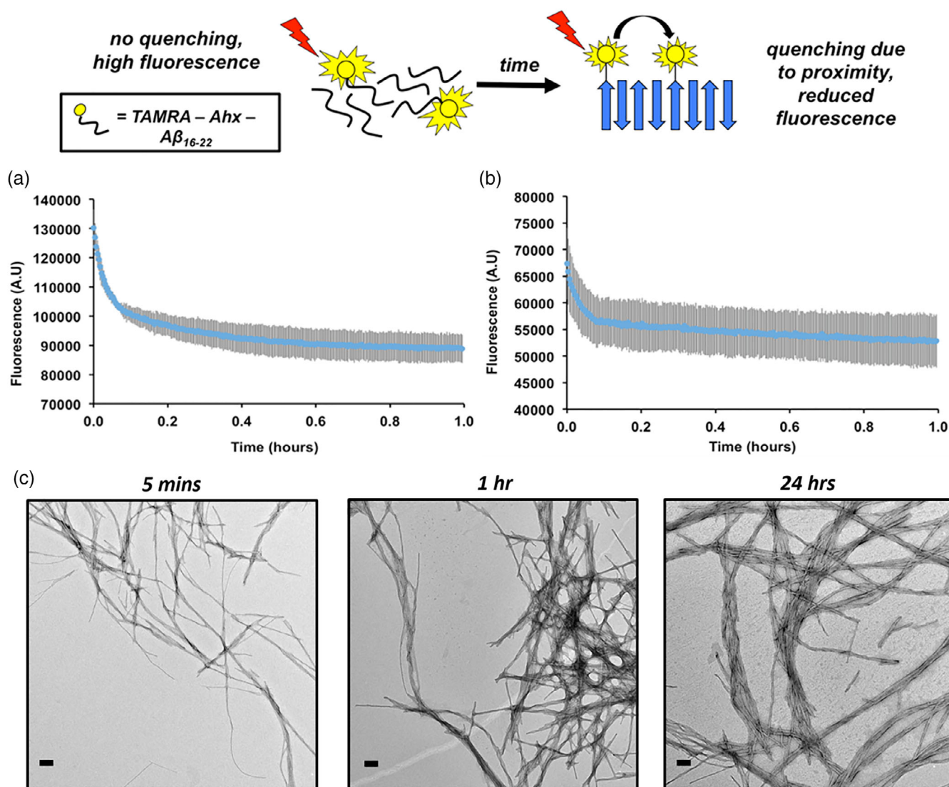
FIGURE 1 Schematic of the fluorescence quenching assay used in this work. As TAMRA-Ahx-A \beta 16-22 is incorporated into the fibrils the fluorophores come into close contact and fluorescence is quenched. The aggregation kinetics of A \beta 16-22 is monitored using fluorescence quenching. At both 40 and 20 \mu M (a and b, respectively), A \beta 16-22 displays two-phase aggregation kinetics with the quenching reaching a plateau after around 1 h (100 mM ammonium bicarbonate buffer pH 7.4 with a final concentration of 2% (v/v) DMSO). In a TEM time course (c), A \beta 16-22 (40 \mu M) forms highly ordered fibril structures within 5 min. Scale bar = 200 nm [Color figure can be viewed at wileyonlinelibrary.com ]
