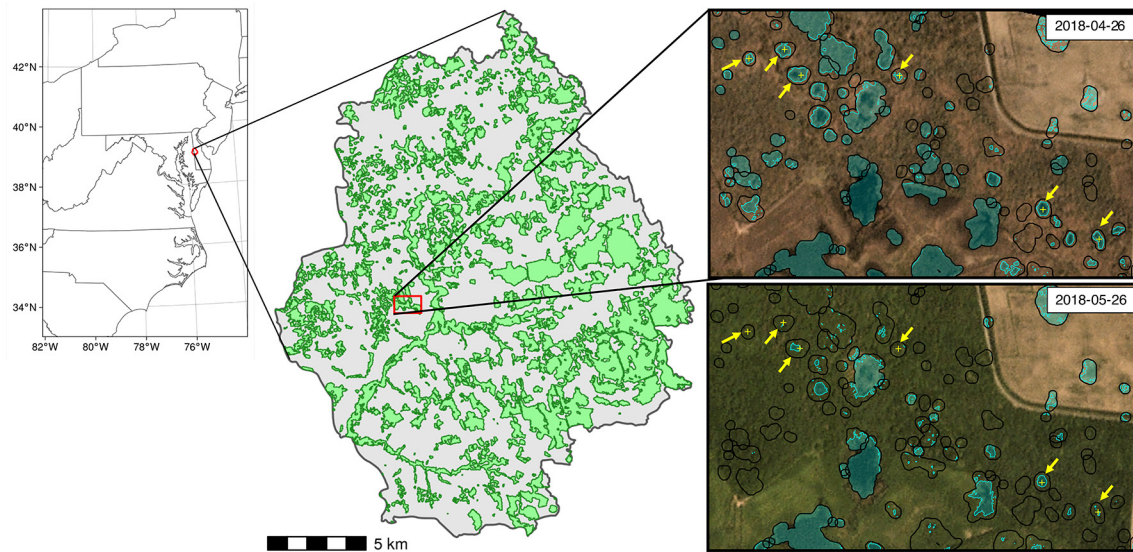
Figure 1. Study area showing location of the Greensboro watershed and forested wetlands. Wetland boundaries, monitoring locations, and surface water classification model predictions for two images are shown over corresponding color-corrected PlanetScope Visual Ortho Scenes (Planet, 2018).
