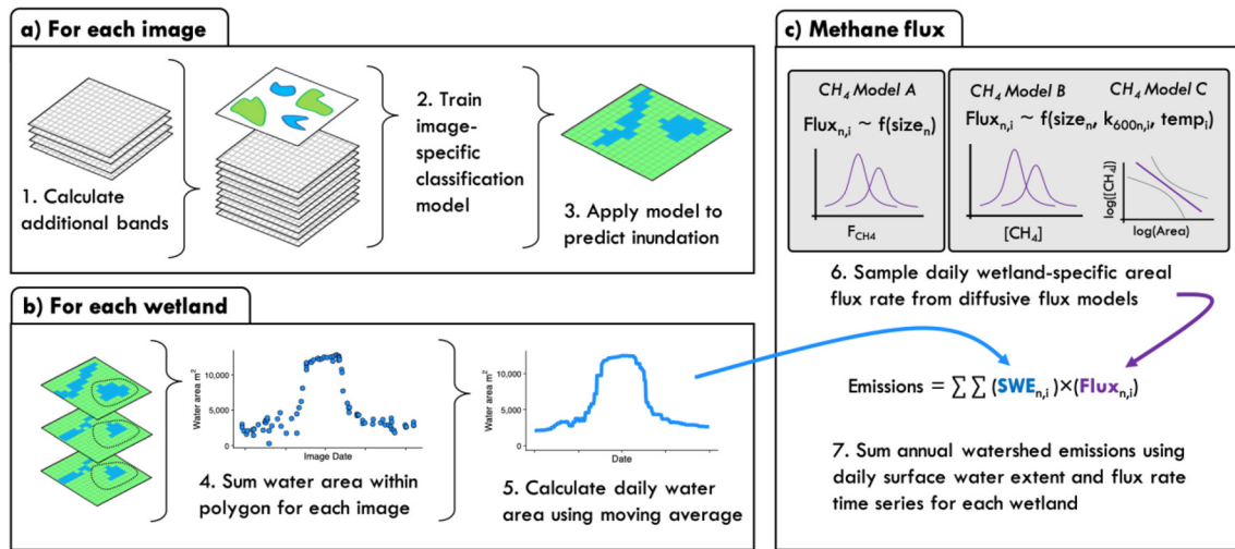
Figure 2. Image classification and emissions model workflow. (a) Image-specific supervised classification models developed using original four bands (R, G, B, and NIR) and derived indices NDVI, NDWI, saturation, chroma, and luminescence. (b) Daily surface water time series derived for each focal wetland from predicted surface water area within each polygon boundary across all images. (c) Methane emissions for each wetland [n] on day [i] derived using semiempirical models to produce annual estimates of basin-wide emissions.
