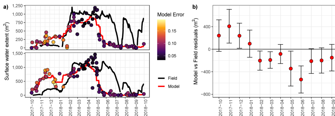
Figure 3. Comparison between inundation time series developed from field monitoring and satellite data. (a) Inundation time series from two wetlands comparing field data and predictions from image-based classification models, along with estimates from individual images (points) shaded by model error rate. (b) Average monthly residuals ( \pm sd) between model predictions of SWE from image classification and field data for all observations across the six wetlands with field water level data.
