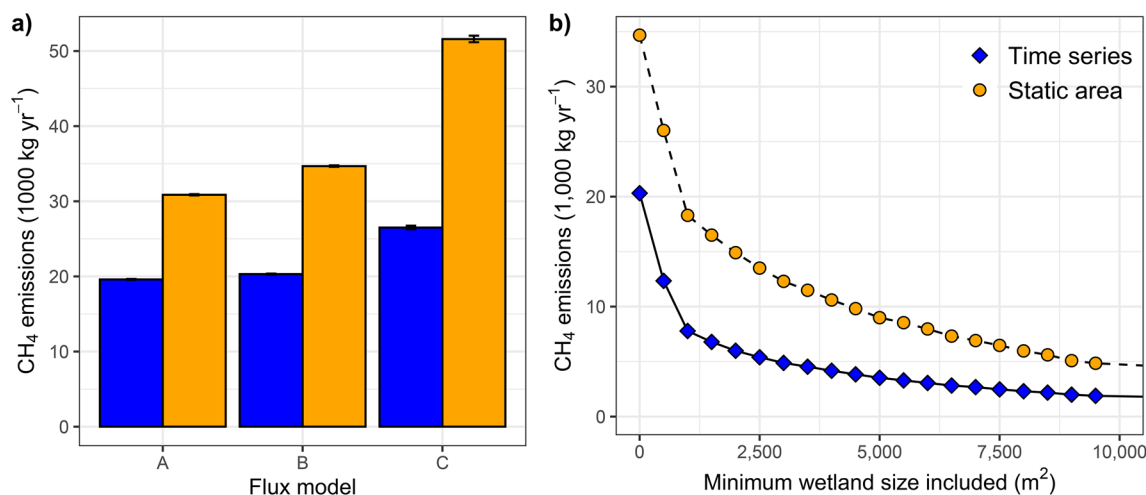
Figure 4. Total annual diffusive methane emissions for focal wetlands calculated using different model assumptions. (a) Total emissions for time-varying (blue) versus static (orange) estimates of SWE using the three semiempirical diffusive flux models described in Section 2.4. Error bars represent 5% and 95% quantiles from 1,000 model iterations. (b) Total emissions for time-varying versus static SWE with different minimum wetland size thresholds.
