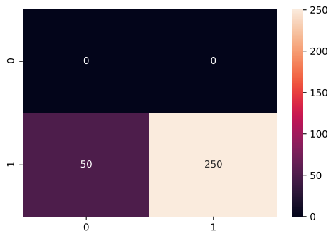
Figure 4: Confusion matrix of Classifier C2
