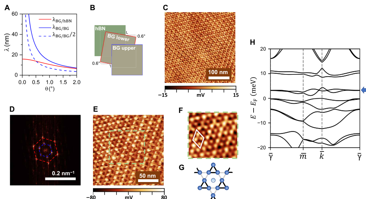
Fig. 4. Kagome-like moiré superstructure in tDBG/hBN. (A) Calculated moiré period of BG/BG and BG/hBN stacks as a function of twist angle. The condition \lambda_{\text{BG/BG}}/\lambda_{\text{BG/hBN}} = 2 is achieved at \theta \approx 0.6^\circ . (B) The sample scheme to realize Kagome-like moiré. The BG/hBN and BG/BG flakes are twisted by 0.6^\circ , but the hBN and the upper BG are aligned. (C) uMIM-Im image. (D) FFT of the image in (C). The dashed hexagons mark the first-order spots of BG/hBN moiré (red) and BG/BG moiré (blue). (E) Detailed uMIM-Im scan of Kagome-like moiré. (F) Low-pass filtered image from the area inside the green square in (E). The unit cell of the Kagome-like moiré is marked with a white diamond. (G) An illustration of a trimerized Kagome lattice resembling the observed moiré. (H) Calculated band structure of the Kagome-like moiré lattice. The high symmetry points refer to that of the Brillouin zone of the BG/BG/hBN superstructure. The blue arrow marks the flat bands near the Fermi level.
