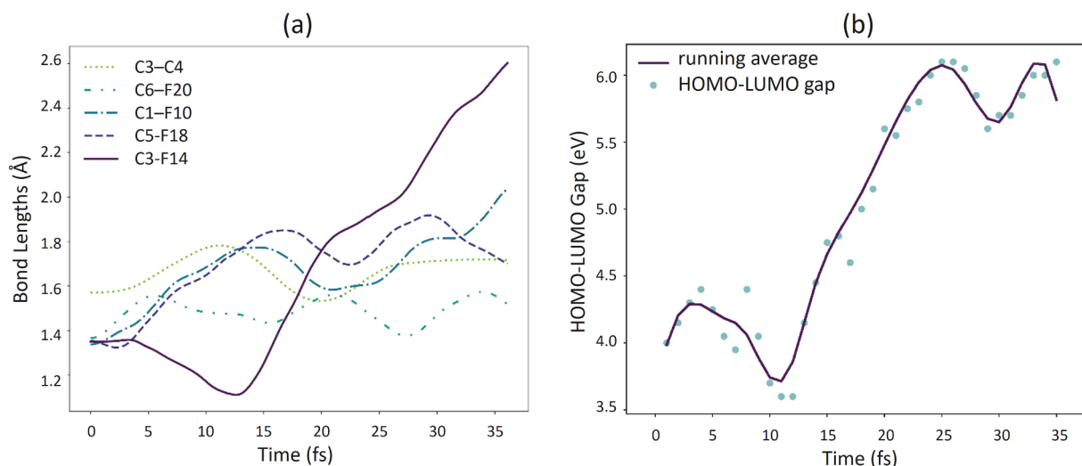
Fig. 3. (a) Variation of selected C–F and C–C bond lengths in PFOA as a function of time (see Fig. 1(a) for atom numbering). After 12 fs, an irreversible elongation of the C3–F14 and C1–F10 bond in PFOA occurs. (b) Variation of the HOMO-LUMO gap of the system as a function of time. At 12 fs, the HOMO-LUMO gap reaches a minimum at which a photo-excited electron transfer occurs, and the C3–F14 bond starts to irreversibly break.
