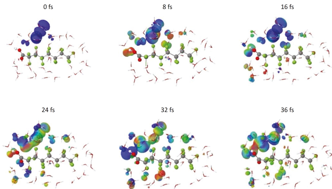
Fig. 5. Variation of the HOMO for PFOA + 43H 2 O molecules as a function of time. As time progresses, charge dynamically transfers from the water to an anti-bonding orbital on PFOA. The C–F bond begins to subsequently destabilize and dissociate as it continues to vibrate dynamically. The positively charged hole remaining in the solvent arising from the afore-mentioned charge-transfer excitation becomes stabilized by the surrounding water molecules.
