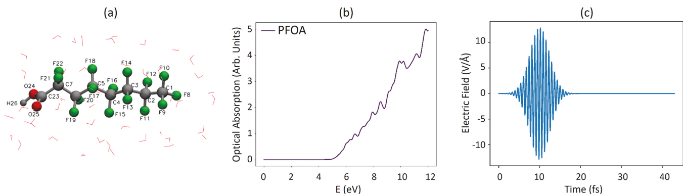
Fig. 1. (a) PFOA molecule surrounded with 43 explicit water molecules (depicted as thin sticks for visual clarity). (b) Optical absorption spectra of PFOA + 43H 2 O molecules. (c) Temporal dependence of the electric field of the applied optical pulse used in our calculations.
