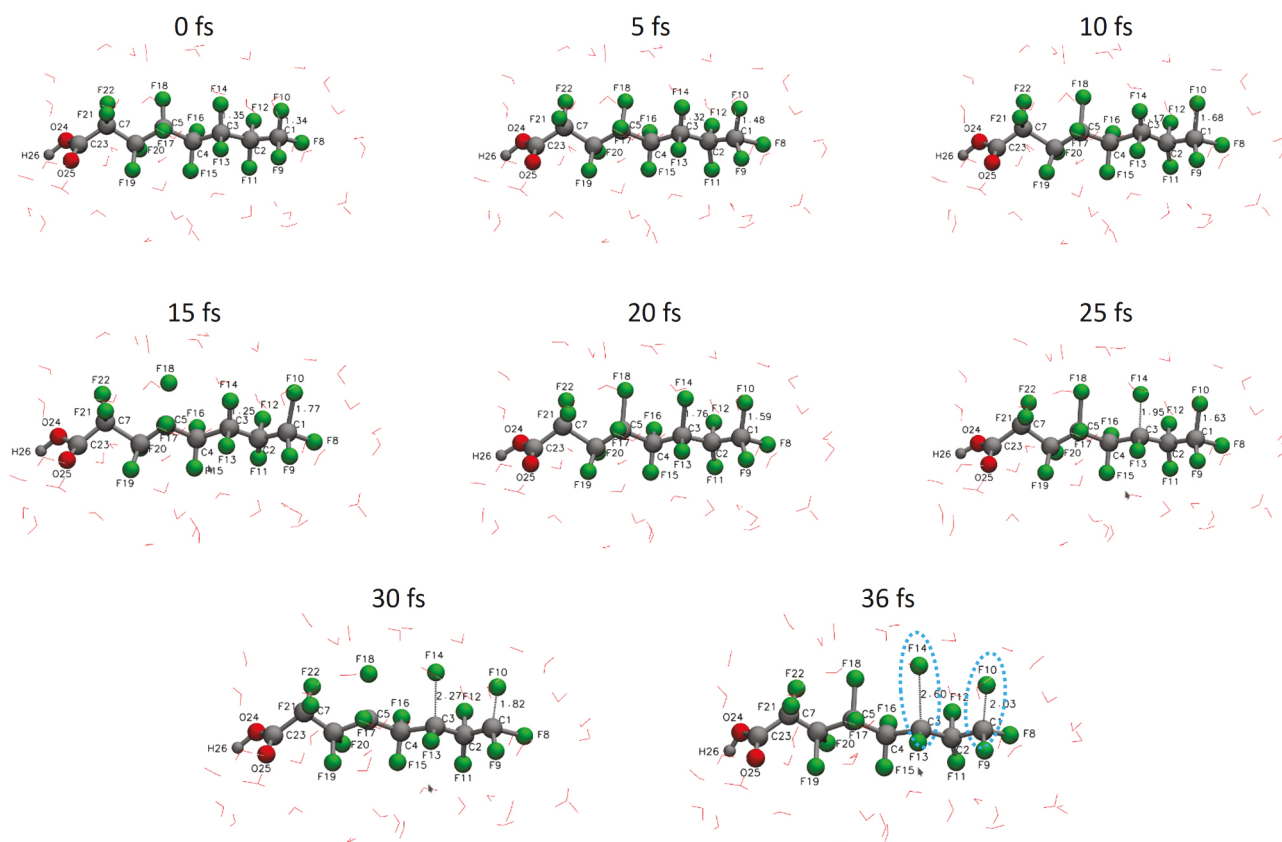
Fig. 2. Variations in the dissociation dynamics of PFOA + 43H 2 O molecules as a function of time. The encircled C3—F14 and C1—F10 bonds in PFOA dissociate at the end of 36 fs.
