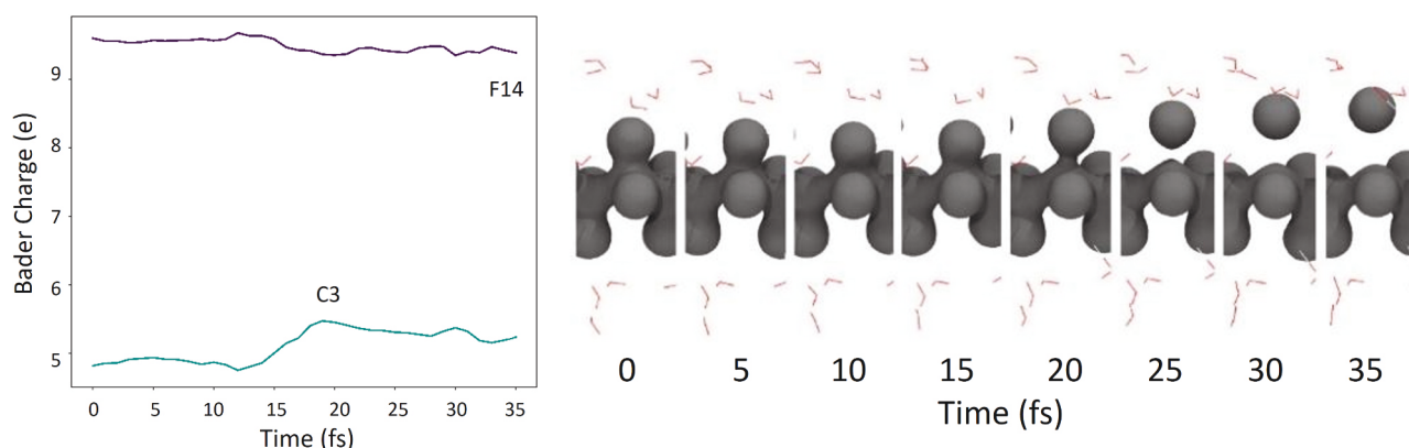
Fig. 4. (left panel) Time-dependent Bader charges for the dissociated C3–F14 bond on PFOA; (right panel) variation of the total RT-TDDFT charge density of PFOA for the C3–F14 bond as a function of time.
