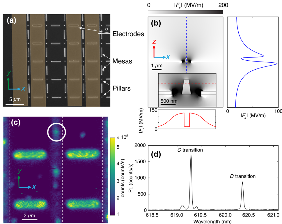
FIG. 1. The device fabrication and characterization. (a) A scanning-electron-microscope image of the fabricated diamond structure and electrodes. The electrodes are highlighted by false-color gold. (b) The simulated electric field magnitude along the x direction ( |F_x| ) for an applied voltage of 200 V across the electrodes. The inset shows a close-up of |F_x| in mesa. The electric fields along the blue and red dashed lines are plotted in the panels to the right ( |F_x(z)| ) and below ( |F_x(x)| ), respectively. (c) The photoluminescence map of the device. One of the \text{Sn-}V^- centers that we study in this work ( E_1 ) is circled in white. The edges of the electrodes are demarcated by white dashed lines. (d) The photoluminescence spectrum acquired from the marked \text{Sn-}V^- center in (c) at zero applied electric field.
