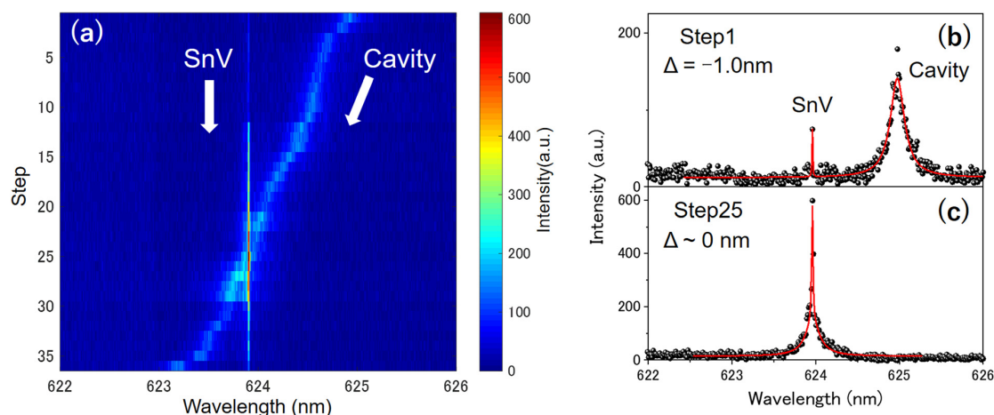
FIG. 2. (a) Color map of low-temperature (4 K) PL spectra taken when the cavity resonance is tuned through the SnV emission by a gas desorption process using a focused laser beam. PL spectrum measured under the detuning (b) \Delta = -1.0 nm and (c) \Delta \sim 0 nm. Red solid lines are fitting curves with multiple Lorentzian peak functions.
