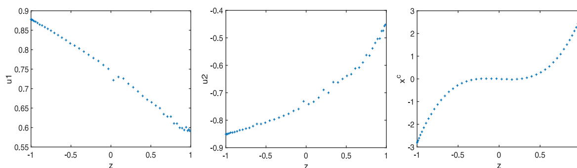
Figure 3. Left to right: u_1 , u_2 , x^c as functions of z . The small zigzags in plots are from numerical error. Numerically to identify these quantities, we look for the biggest jump between two adjacent grid points. This procedure brings some error and is not easily eliminated by adopting another numerical solver for the conservation law.
