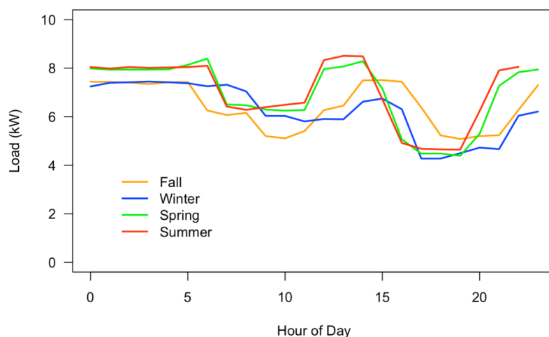
Figure 1. Averaged hourly electrical load profiles of a container farm in Whitehorse, Yukon for fall (September–November), winter (December–February), spring (March–May), and summer (June–August). Electricity use is greatest overnight along with a midday peak when all loads (lighting, heating/cooling/ventilation, dehumidification) are operating. Reductions in electric use occur in the mid-morning hours, which can be attributed to reduced heating, cooling, and dehumidification as well as late afternoon and evening hours when lighting is turned off. Summer electricity use is generally highest, given substantial cooling required to exhaust waste heat from operating electric loads, which are nearly sufficient to heat the opaque container in the winter.
