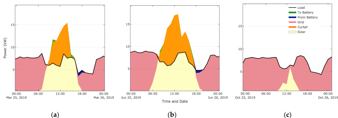
Figure 2. Modelled electric profiles resulting from operating the optimized solar and storage system with the collected container farm load data for three representative seasonal periods: (a) Spring, (b) Summer, and (c) Fall. In spring and summer, a small amount of excess solar was used to charge the battery in the afternoon and the solar day of the battery was smaller amount of charging necessary during the summer given that more solar energy is available from day to day generation and charging the battery and charging the battery was curtailed. When the battery had energy in storage in the early evening hours, the battery was discharged in the early evening hours. In late fall and winter, solar energy output was less than the container farm load.
