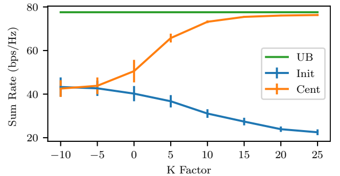
Fig. 7: Optimizing positions improves capacity for LOS dominant channel having a large K-factor. Simulation is done for the placement in Fig.6a and includes localization errors and channel estimation errors.
