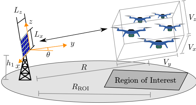
Fig. 4: In the simulation setup, the UAVs are initialized in a rectangular area. The GS is tilted towards the swarm.
