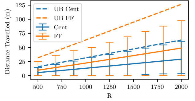
Fig. 10: The mean distance traveled by the swarm. The error bars represent the range.
