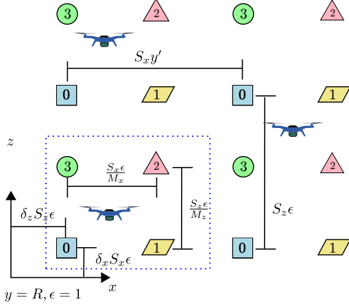
Fig. 2: An illustration of the set \mathcal{P} for a swarm placed on the same plane at y = R for a 2 \times 2 URA. The numbered colored shapes identify different positions. Each UAV needs to occupy a different position to maximize capacity.
