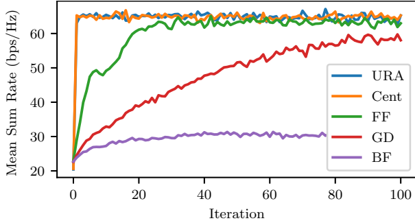
Fig. 9: The sum rate of distributed approaches under practical disturbances.
