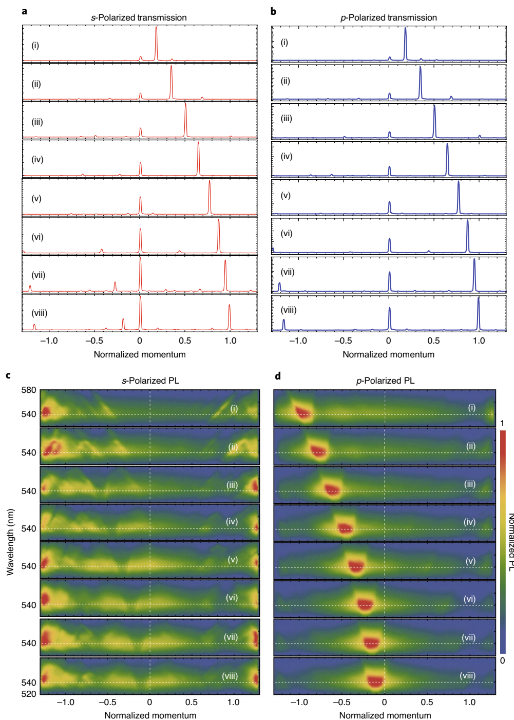
Fig. 2 | Directional metasurface transmission and emission. a, b, s - and p -polarized transmission through eight distinct metasurfaces as a function of the normalized in-plane momentum ( k_{\parallel}/k_0 ). The metasurface design deflects a normally incident beam ( 0^\circ ; k_{\parallel} = 0 ) to a transmitted beam ranging between k_{\parallel}/k_0 = 0.17 ( 10^\circ in air; (i)) to k_{\parallel}/k_0 = 0.98 ( 80^\circ in air; (viii)) using a linear phase profile. Comparing the specular transmission ( k_{\parallel}/k_0 = 0 ) to the deflected beam ( k_{\parallel}/k_0 > 0 ) illustrates the relative efficiency of the metasurface (see for example Fig. 4a). c, d, s - and p -polarized PL as a function of wavelength ( y axis, 520–580 nm) and normalized in-plane momentum ( k_{\parallel}/k_0 ; x axis) for the eight different metasurfaces (one in each panel, (i)–(viii)). Data in each panel have been normalized such that the maximum PL in each plot is equal to unity. The p -polarized PL peak is shifted in momentum space from -1 to 0 based on the metasurface design.
