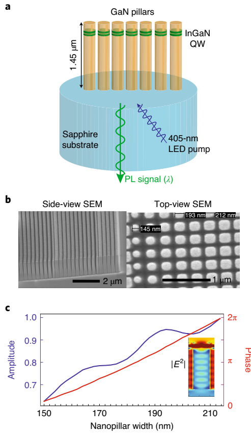
Fig. 1 | Metasurface schematics and design. a , Illustration of the GaN nanpillar system with InGaN multiple QWs (green) grown on a GaN base layer on a double-side polished sapphire substrate. In our experiments, samples are optically pumped using a 405-nm LED and emitted PL is collected from within the substrate using momentum-resolved (that is, Fourier) imaging techniques. b , Scanning electron microscopy (SEM) images of a GaN metasurface showing the high-aspect-ratio nanpillars formed with a well-defined size gradient only along the x direction. c , The phase (red, right axis) and normalized amplitude (blue, left axis) of the light emitted into the substrate from the point in-plane ( x, y ) electric dipole embedded in the GaN nanpillar as a function of the nanpillar width. The inset shows a characteristic electric field intensity ( |E^2| ) profile of the excited mode by the point dipole with red (blue) representing maximum (minimum) in field intensity.
